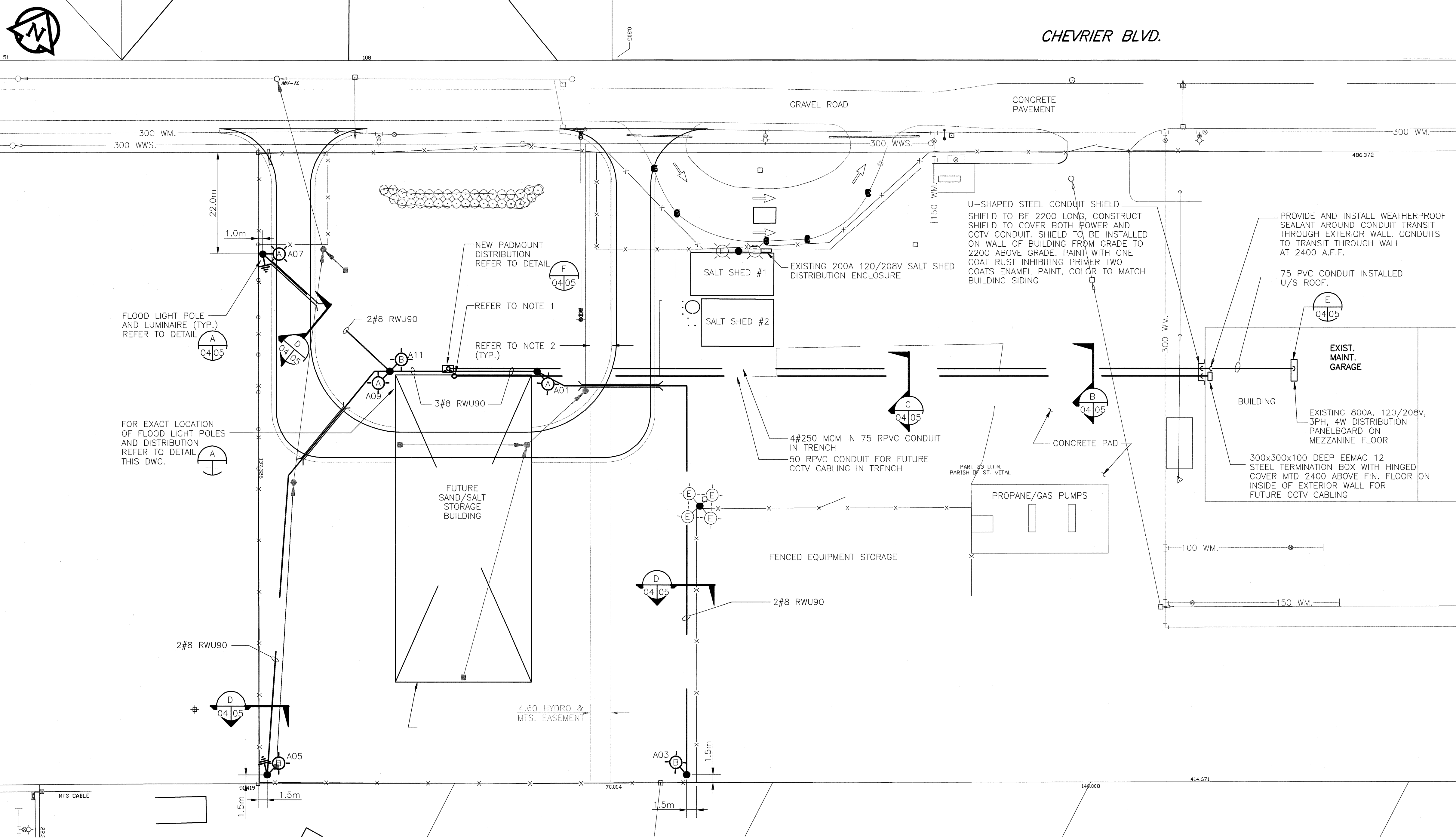
1 PARTIAL SITE PLAN 1:500
