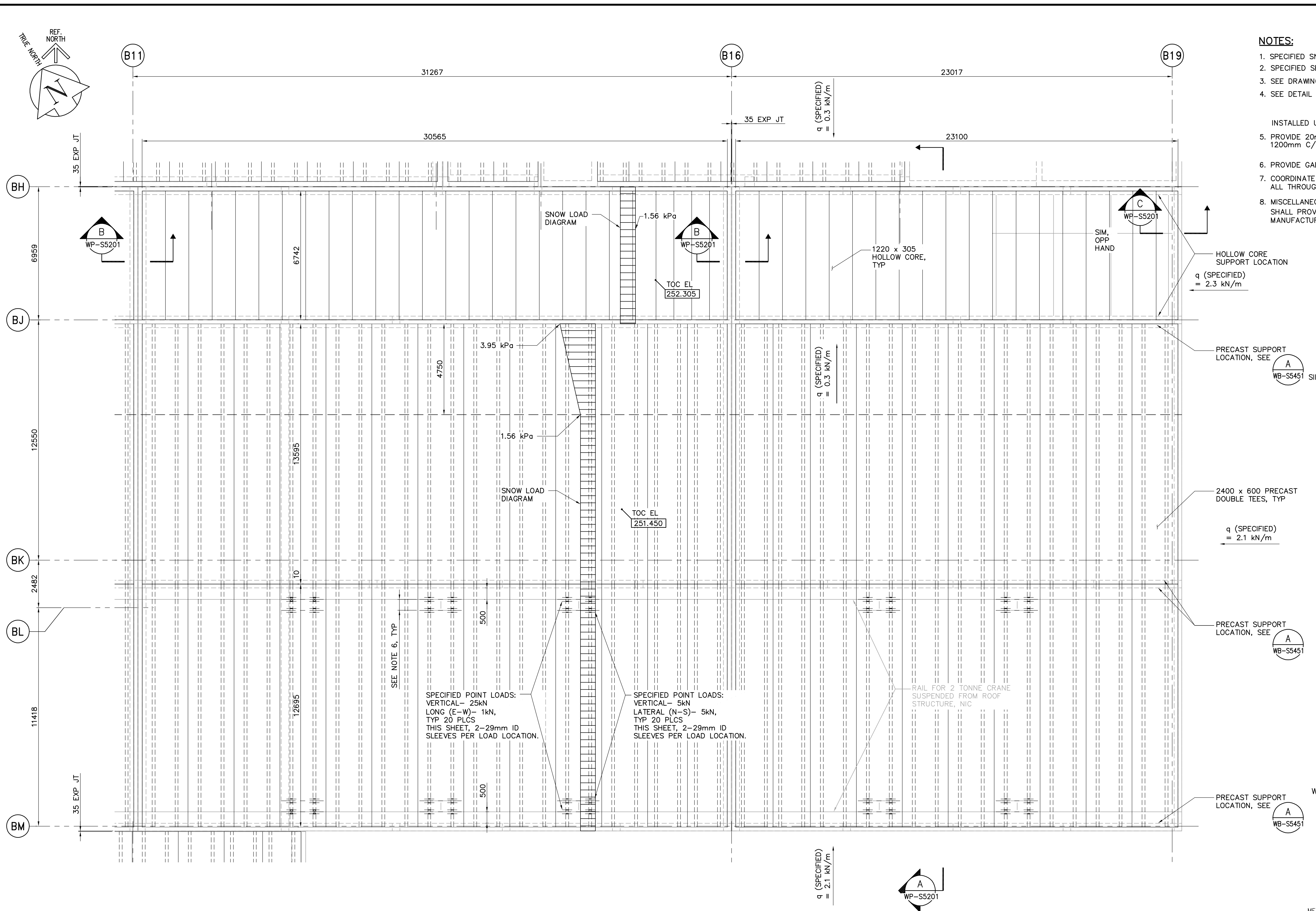
ROOF PLAN 1:100
