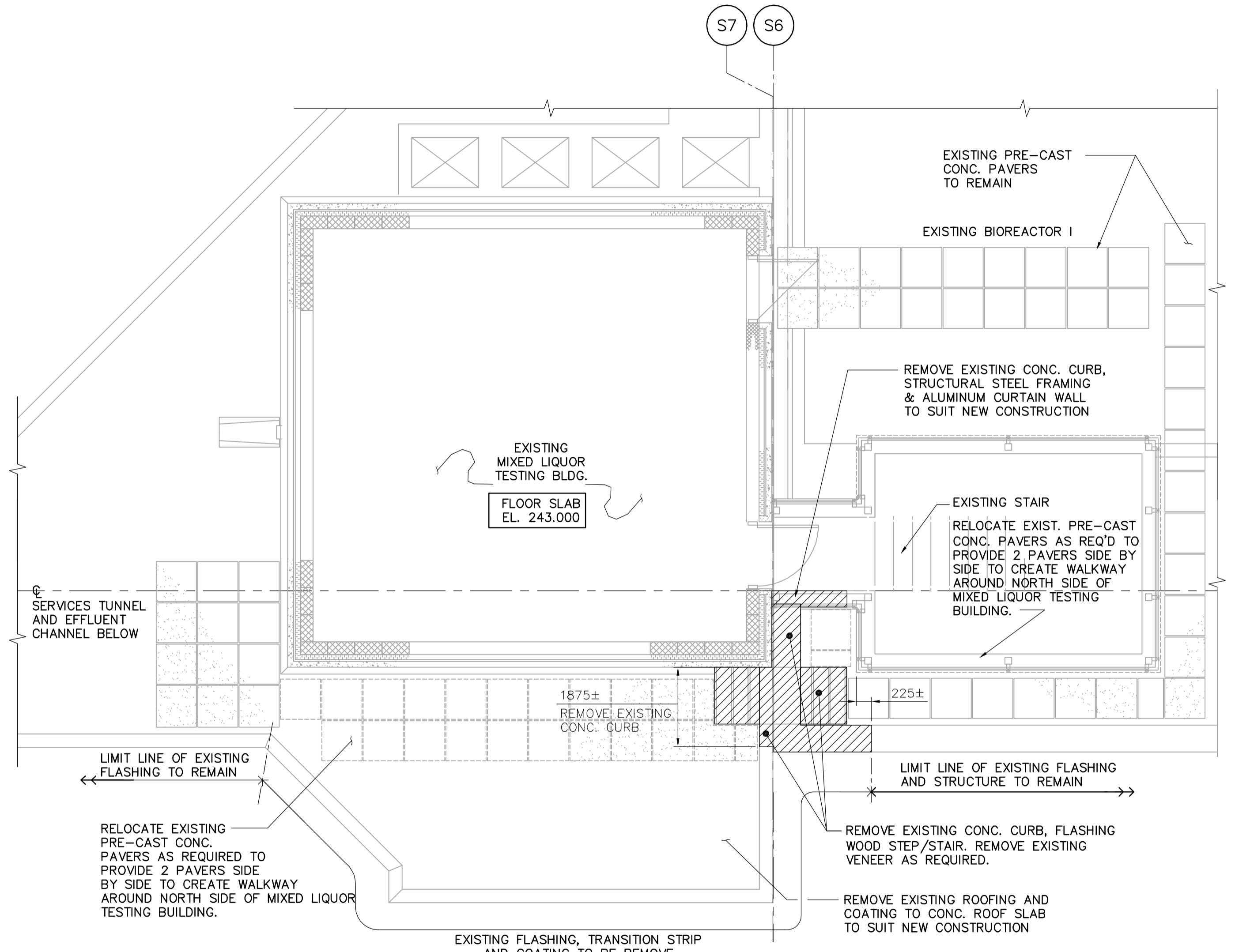
2 MAIN FLOOR DEMOLITION PLAN SA6.01 SCALE 1:50
