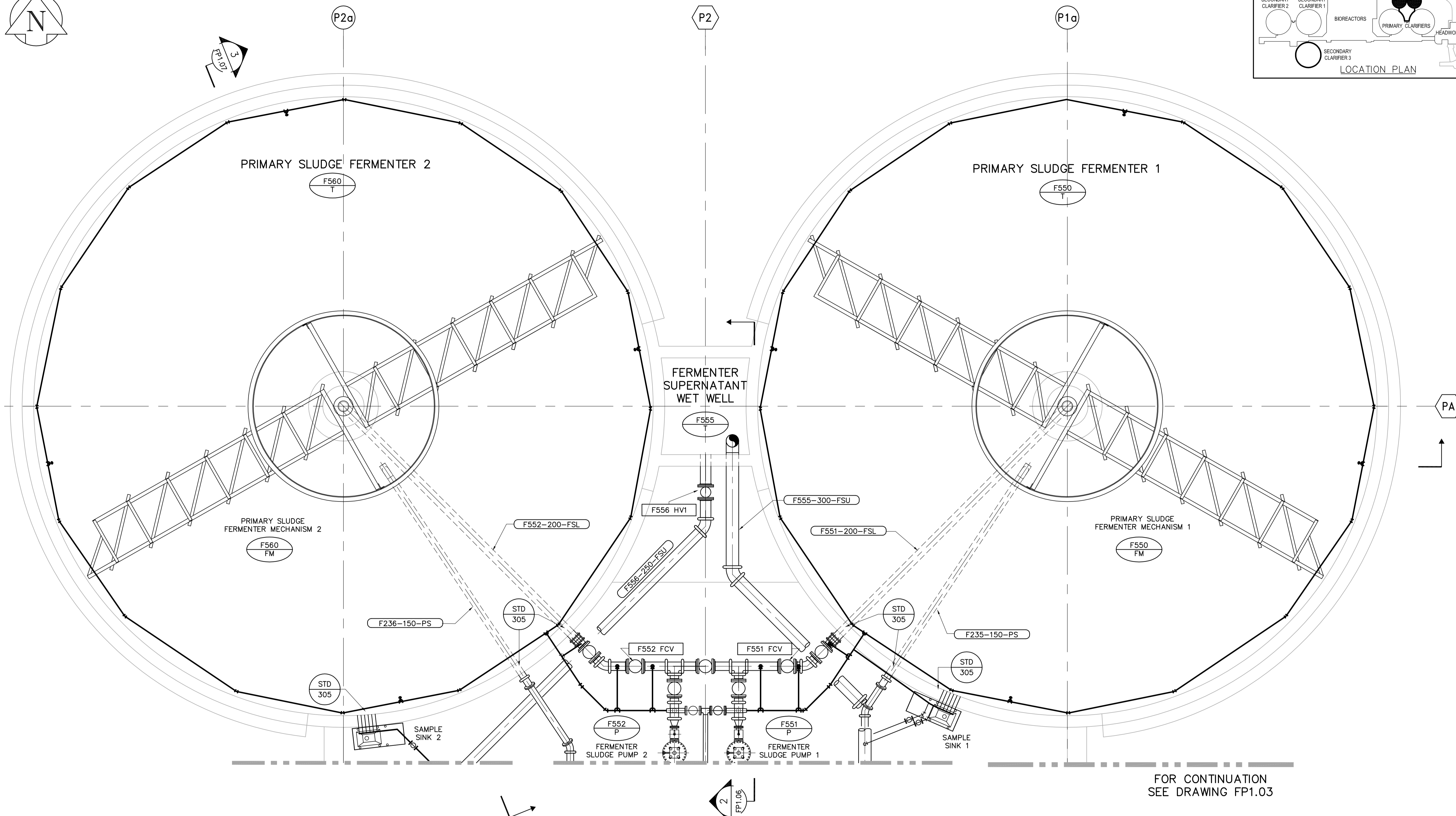
LOWER LEVEL PLAN - PRIMARY SLUDGE FERMENTERS 1 & 2 1:50
