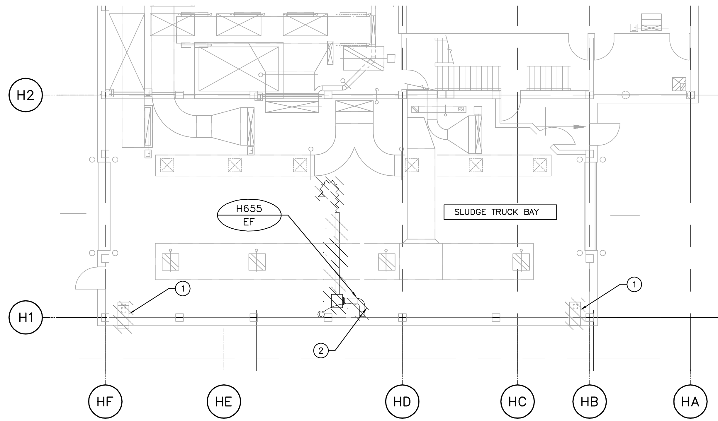
EXISTING MAIN FLOOR VENTILATION DEMOLITION PLAN SCALE: 1:100
