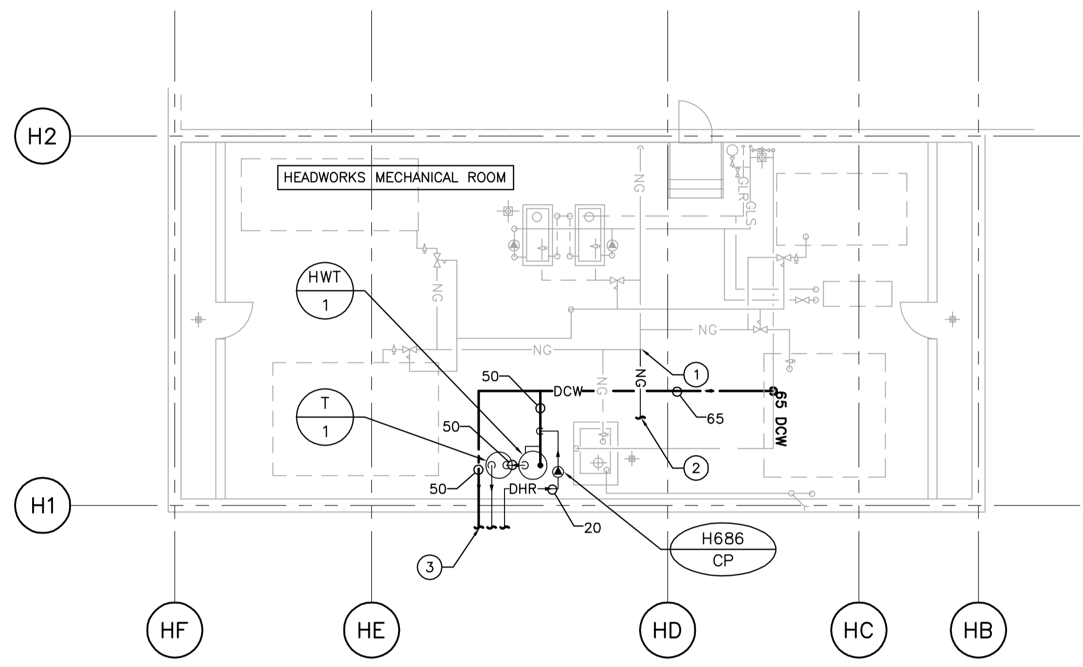
UPPER LEVEL - PLUMBING PLAN SCALE: 1:100
