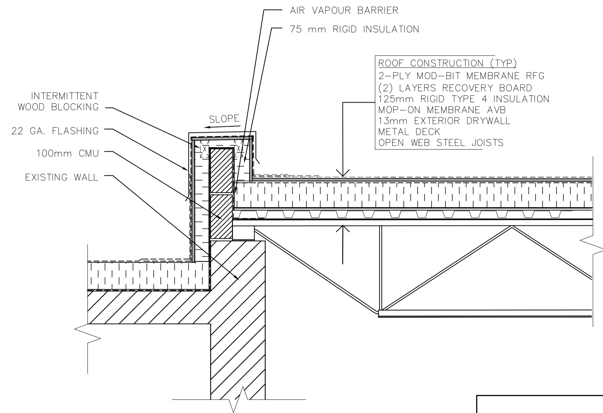
3 ROOF TIE-IN SECTION DETAIL SA3.01 1:10
