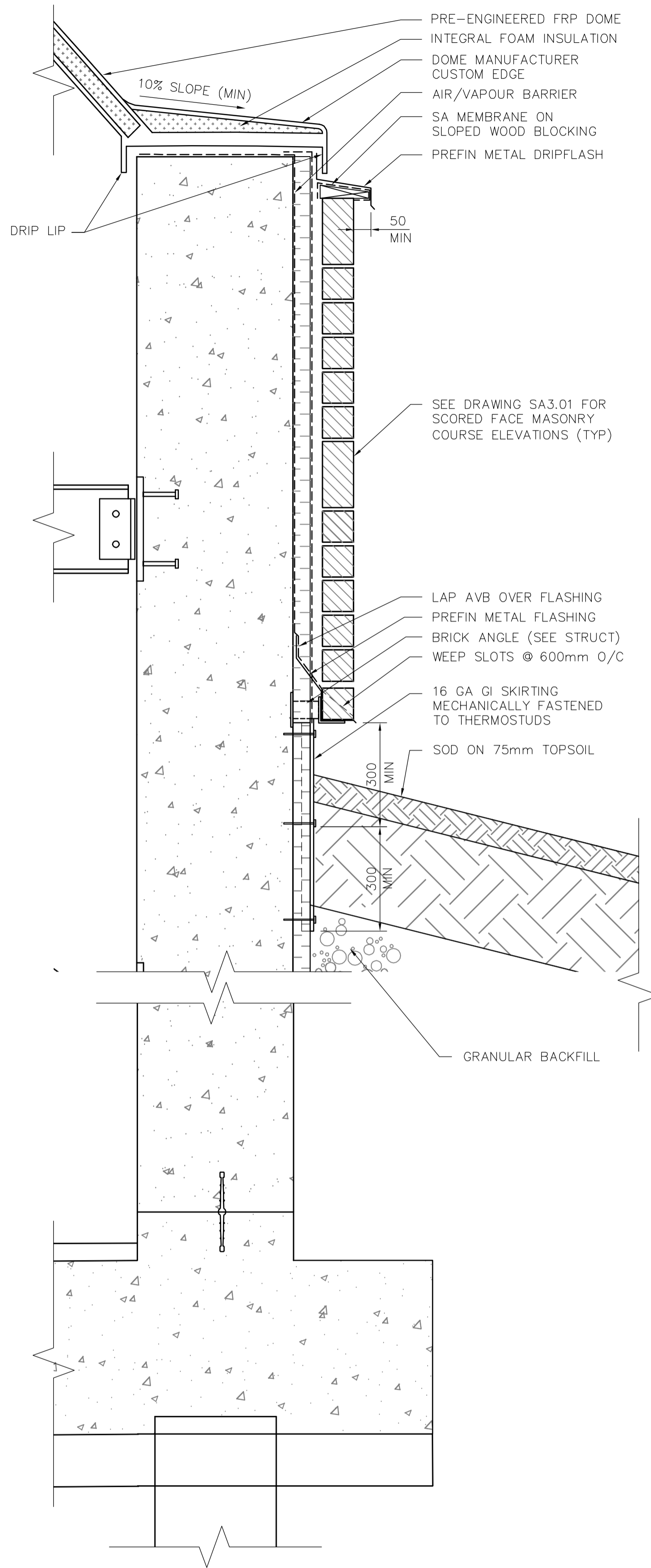
2 CLARIFIER WALL SECTION (TYP) SA3.01 1:10
