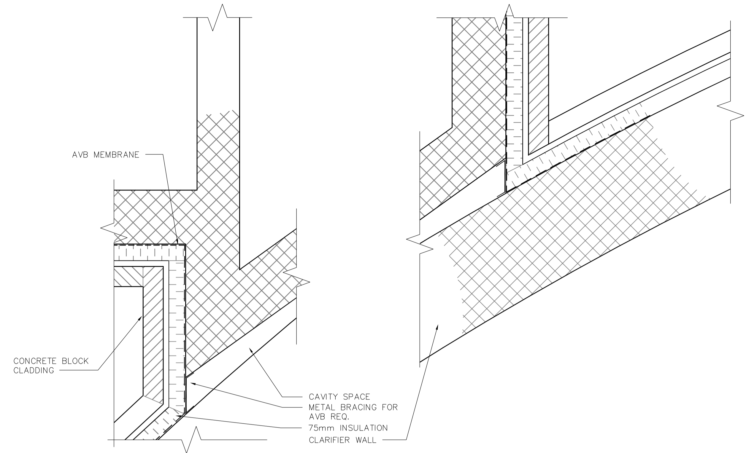
4 BUILDING TIE-IN PLAN DETAIL SA1.02 1:10
