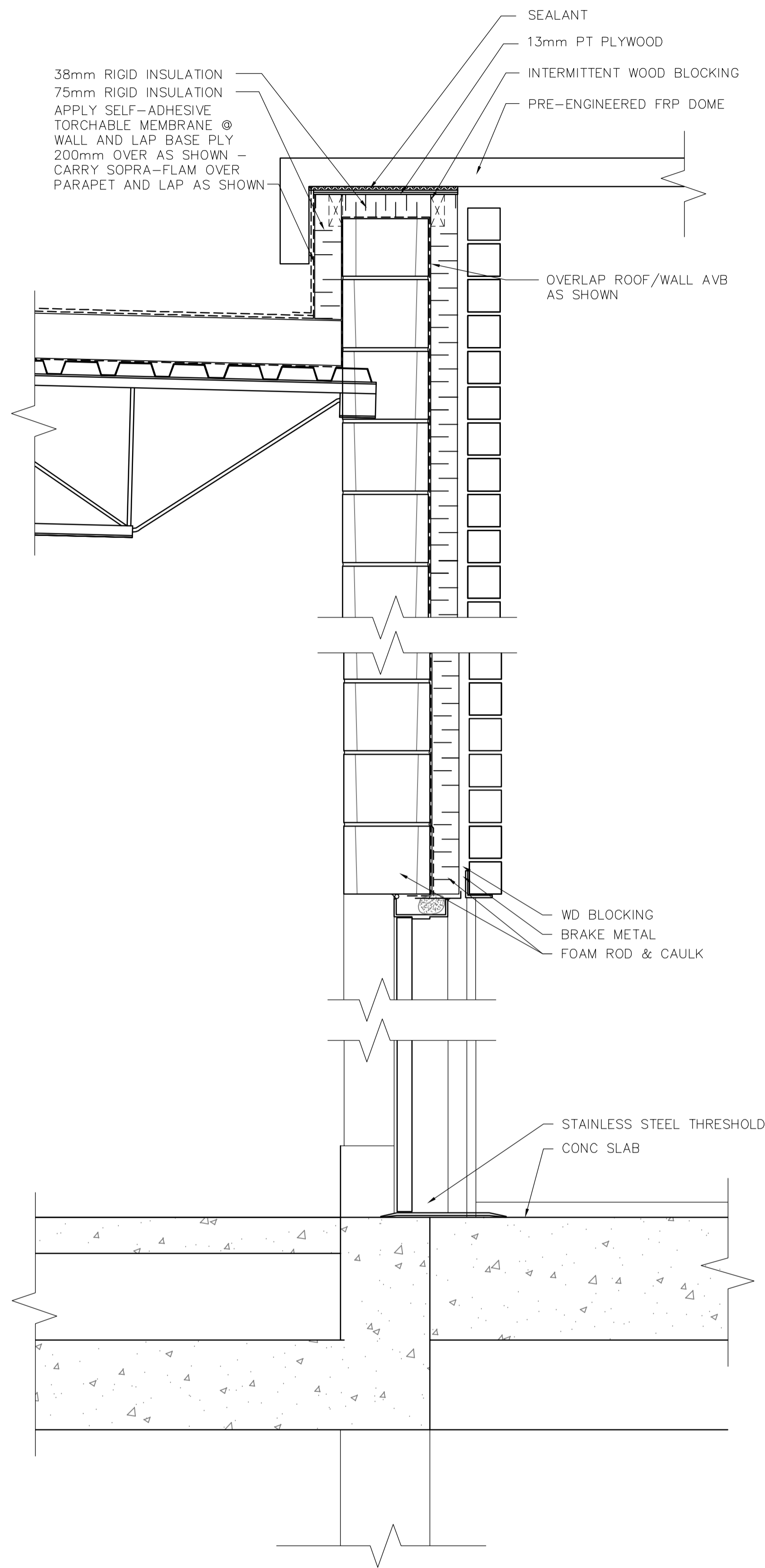
1 WALL SECTION AT DOORS SA3.01 1:10
