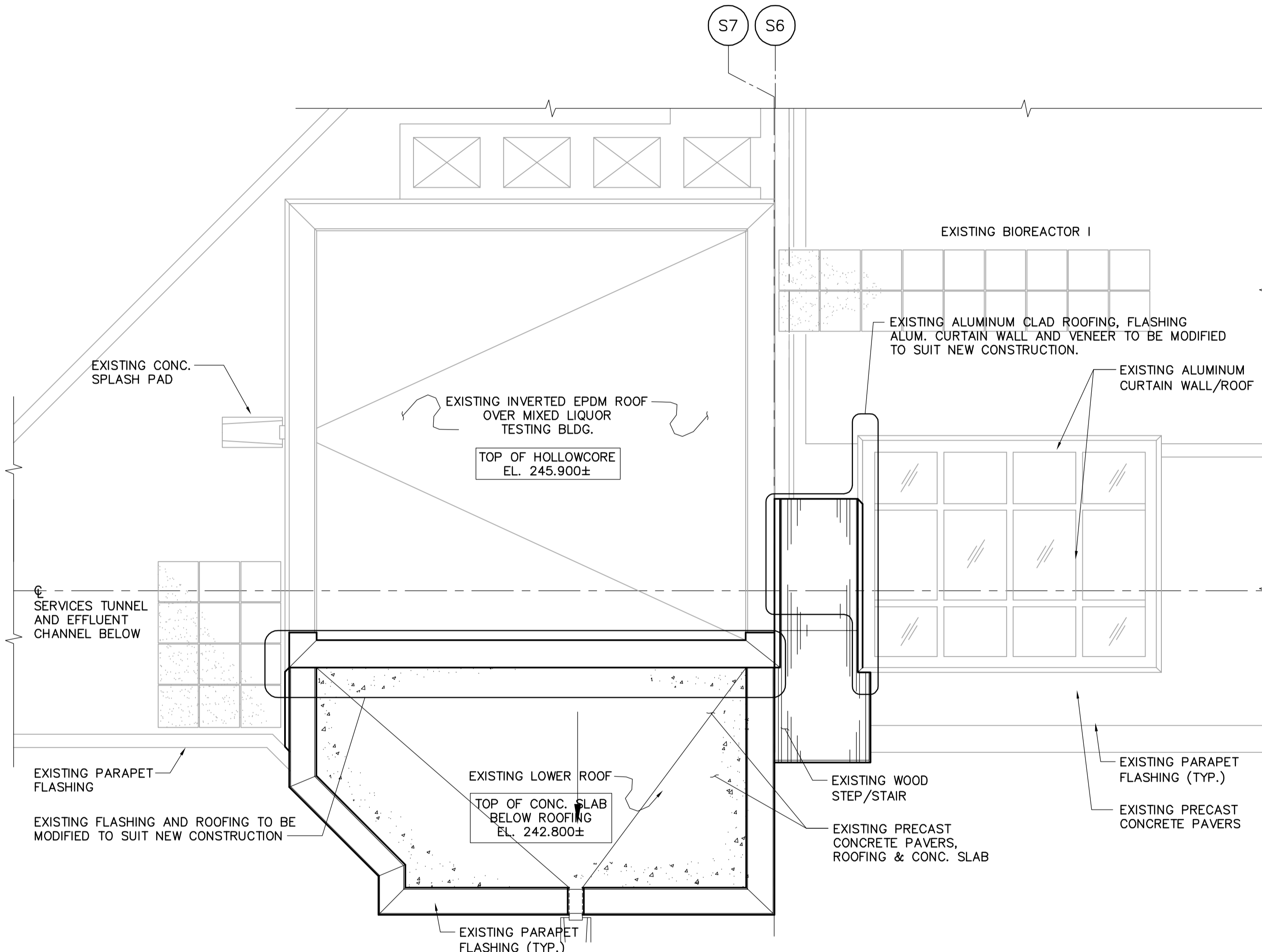
1 ROOF DEMOLITION PLAN SA6.01 SCALE 1:50
