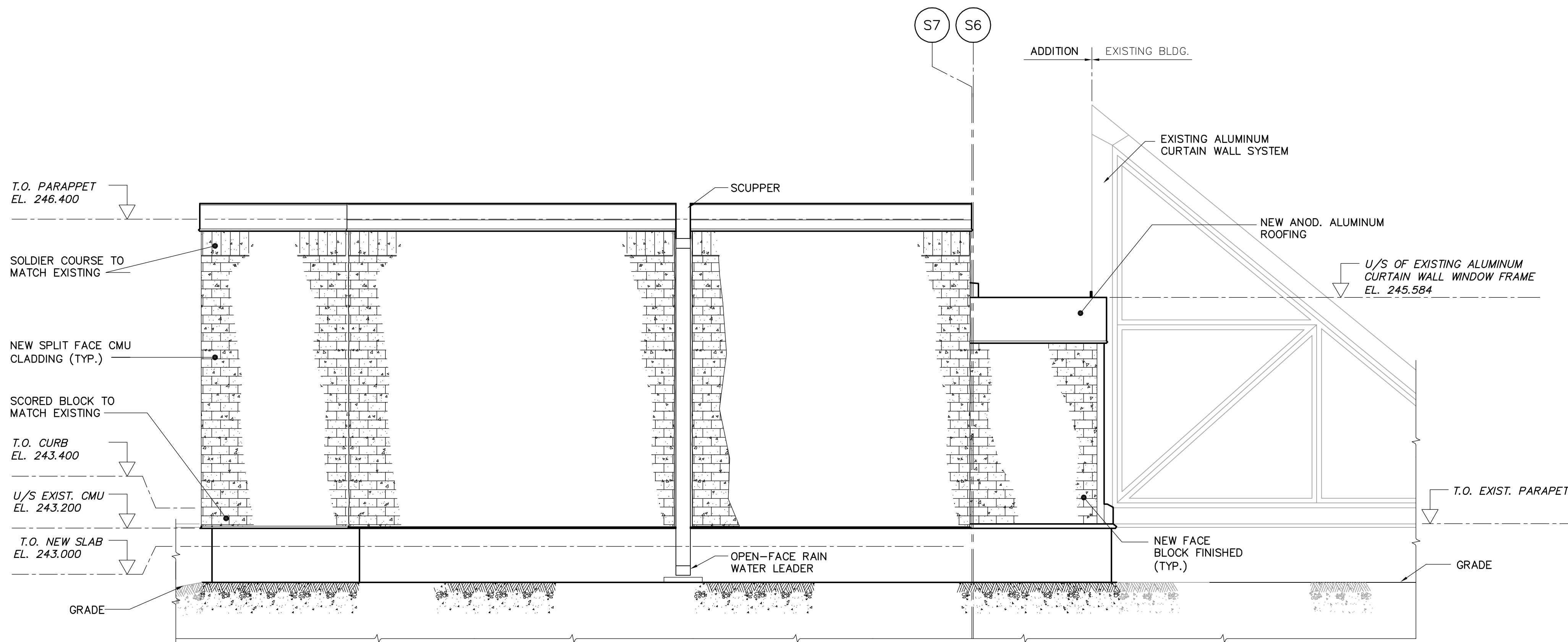
1 SOUTH WALL ELEVATION SA7.01 SCALE 1:30
