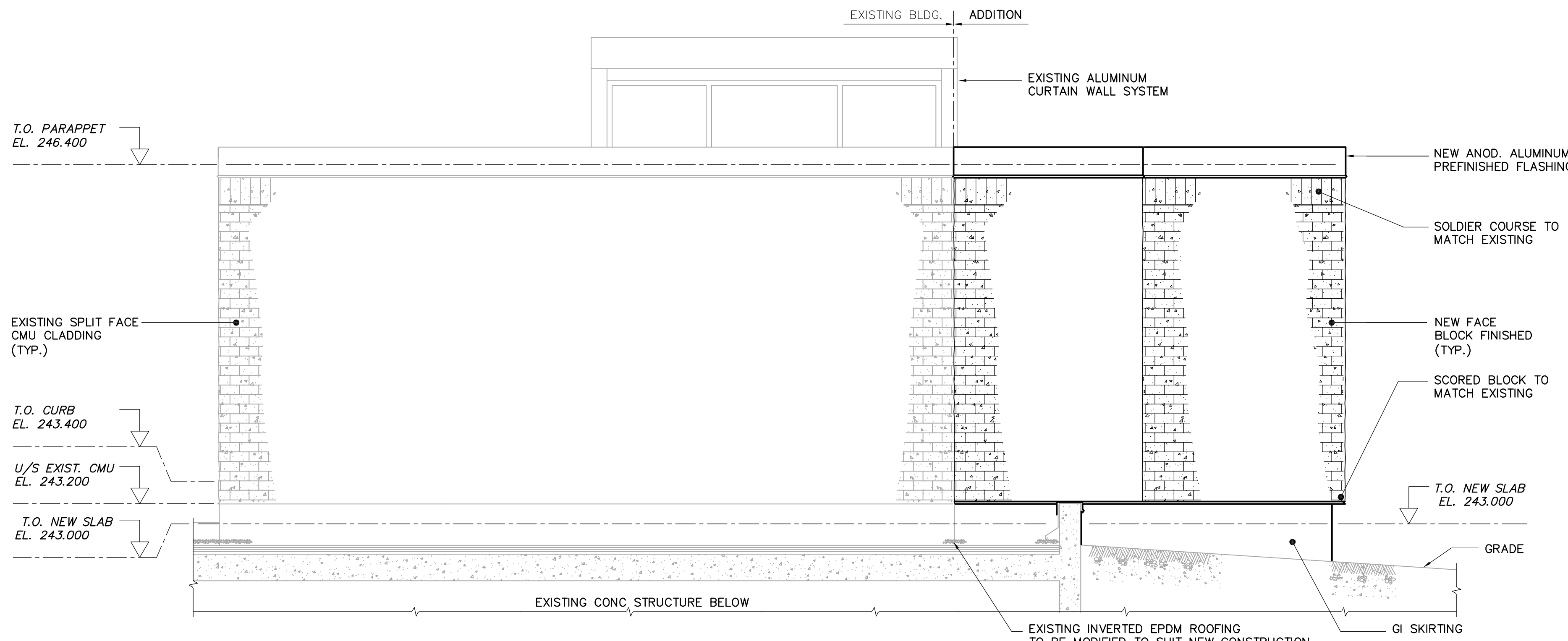
2 WEST WALL ELEVATION SA7.01 SCALE 1:30
