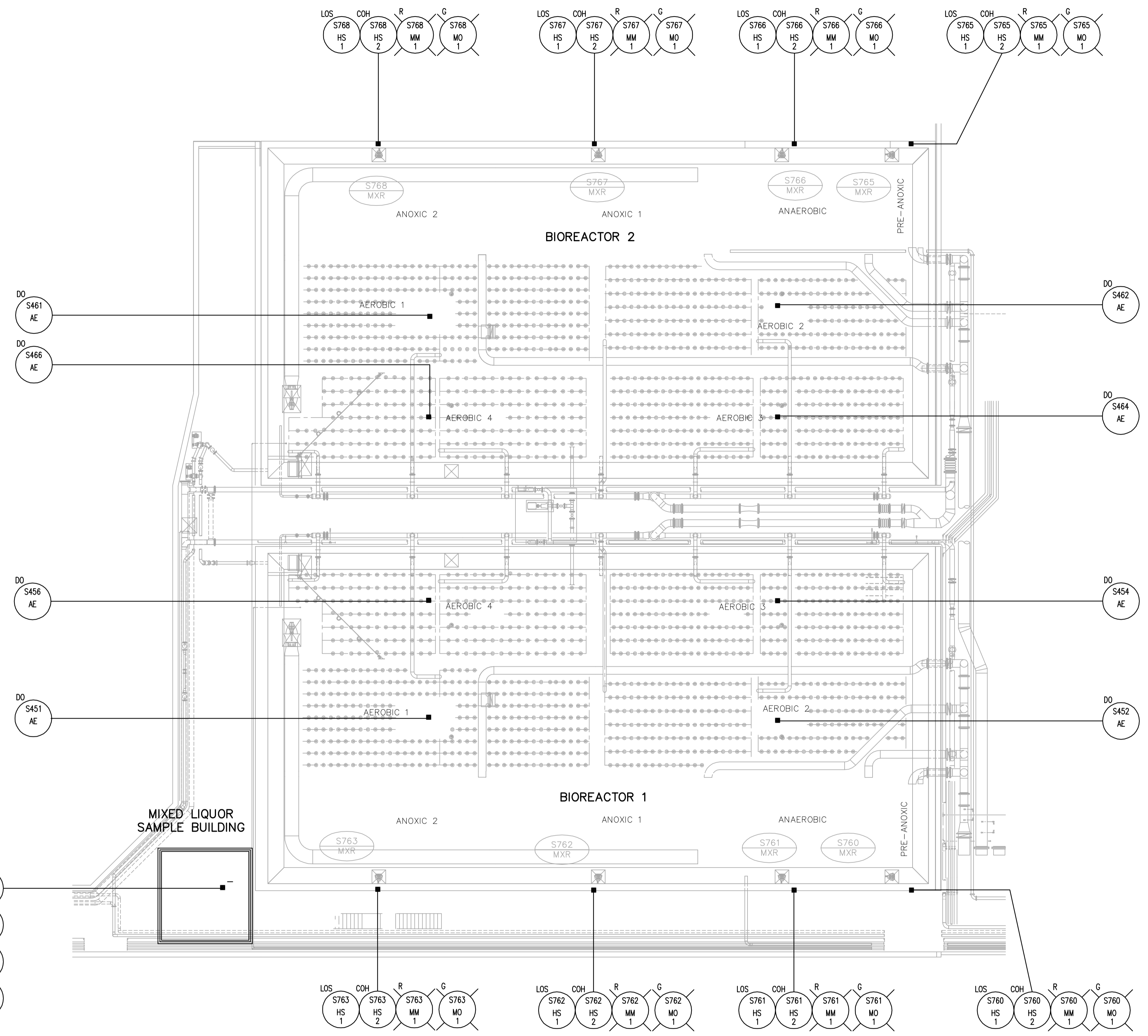
LOCATION PLAN - BIOREACTORS 1 & 2 1:100
