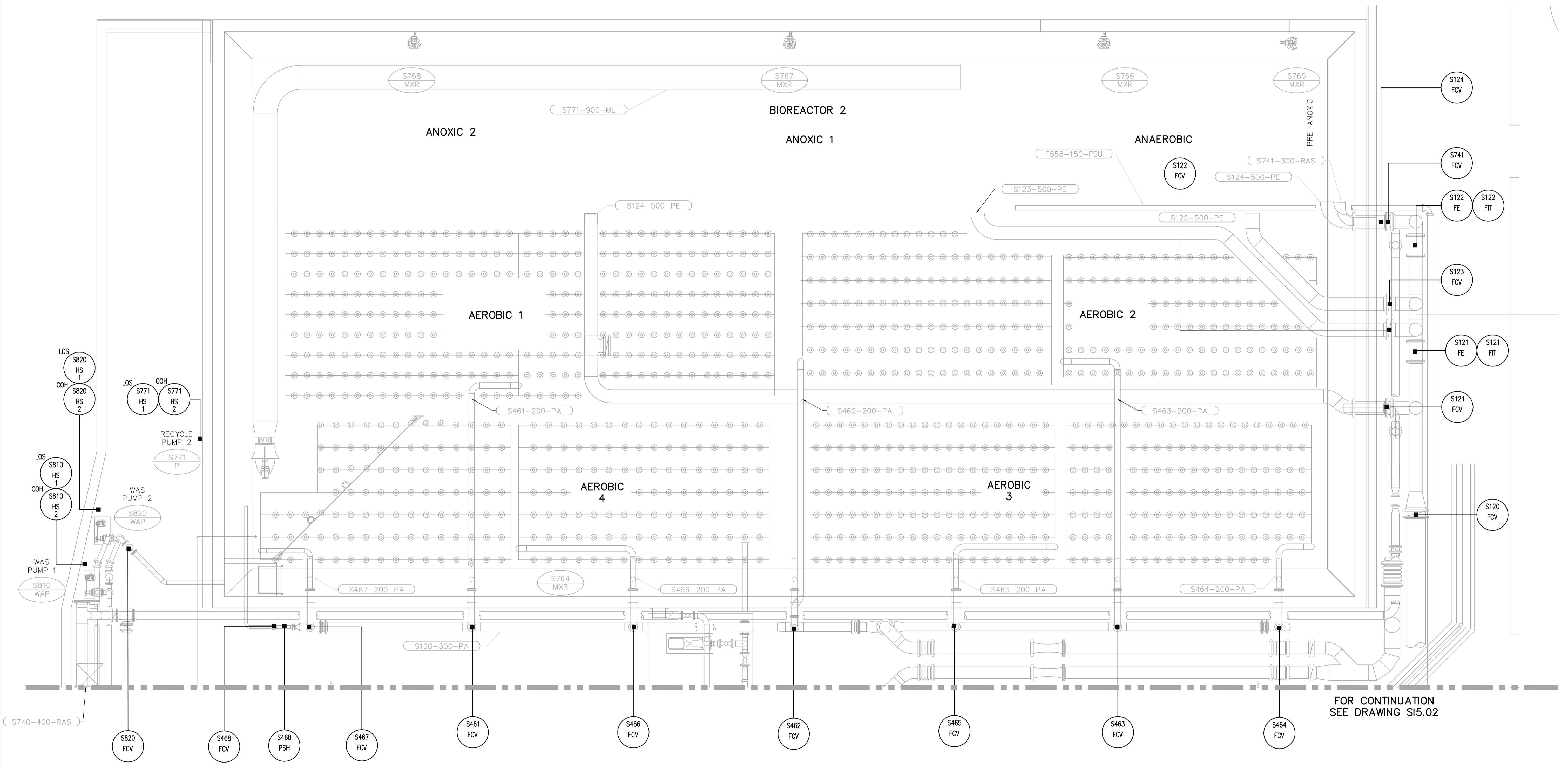
LOCATION PLAN - BIOREACTOR 2 1:75
