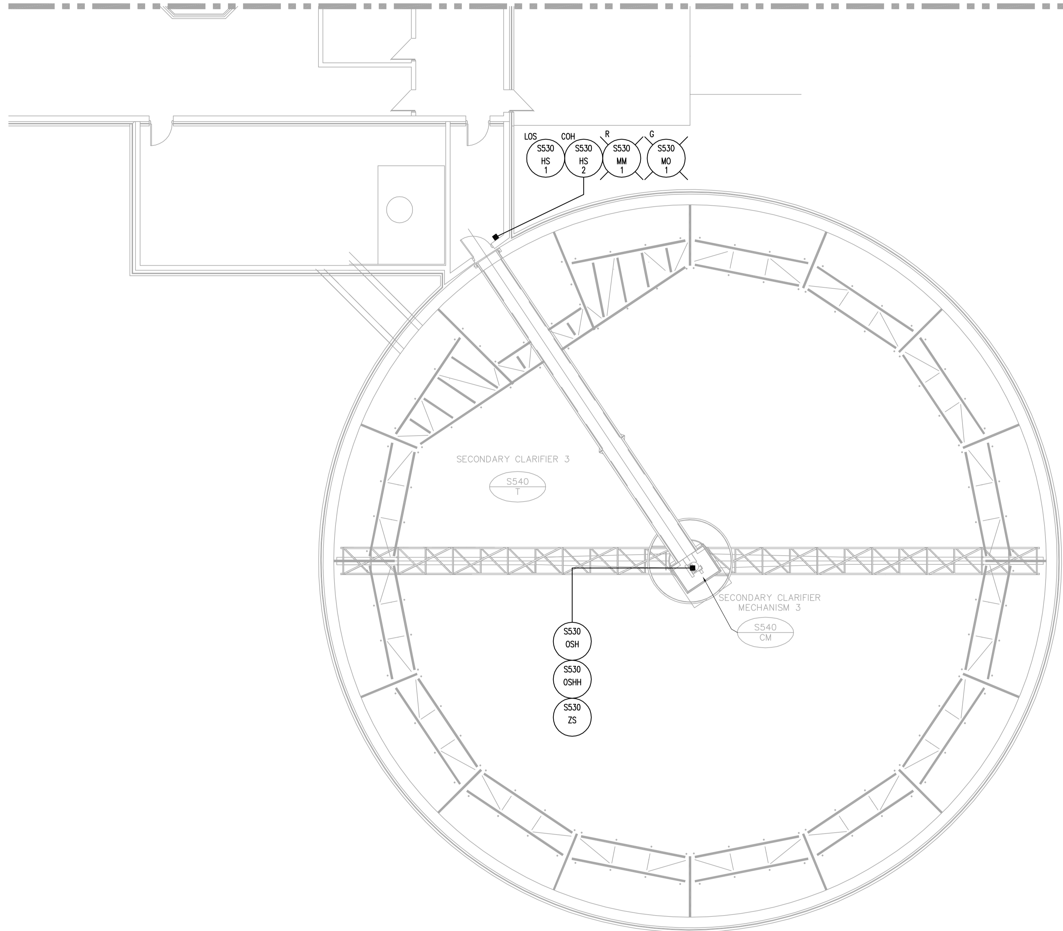
— UPPER LEVEL LOCATION PLAN — SECONDARY CLARIFIER 3 1:100
