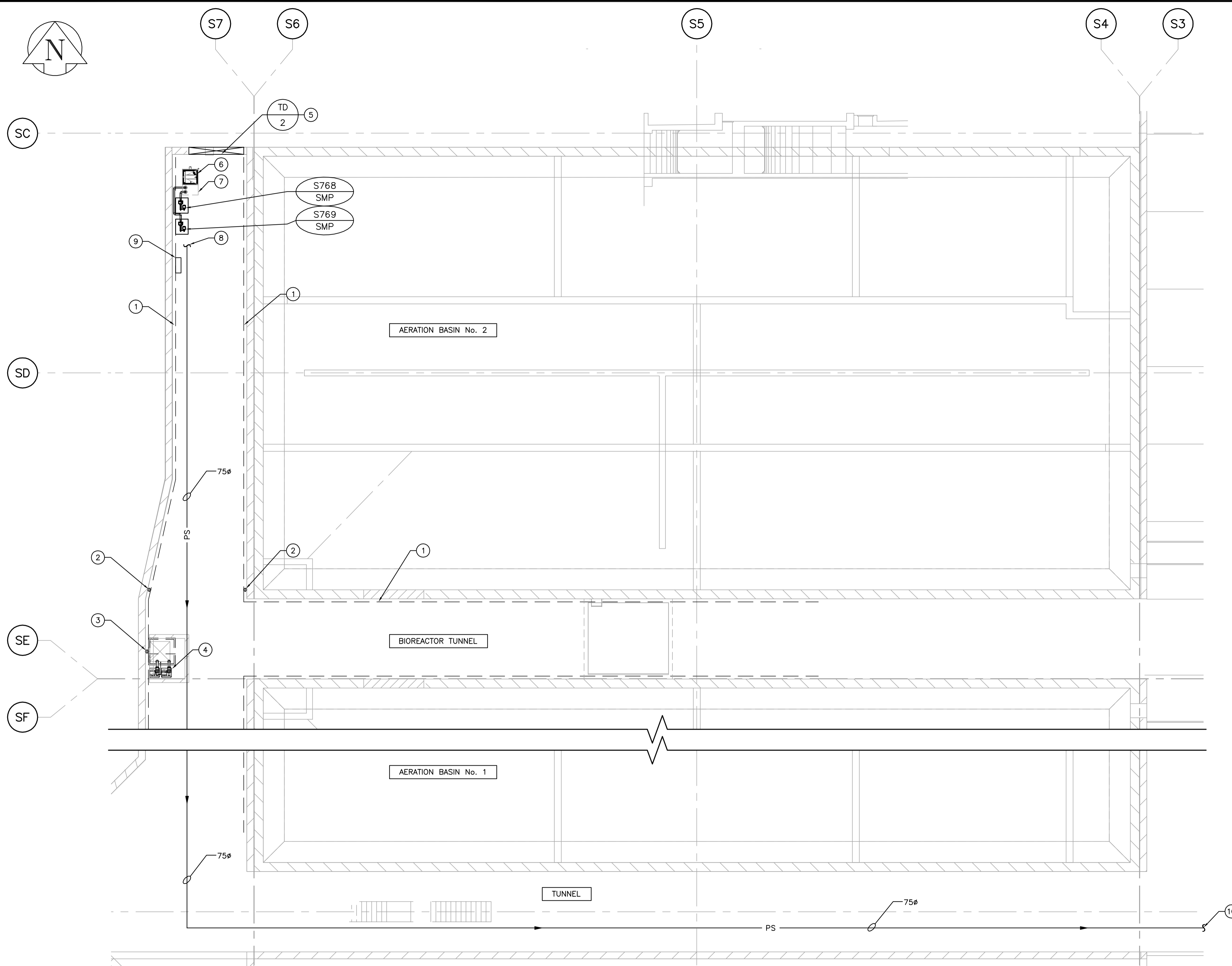
LOWER LEVEL – MECHANICAL PLAN SCALE: 1:100
