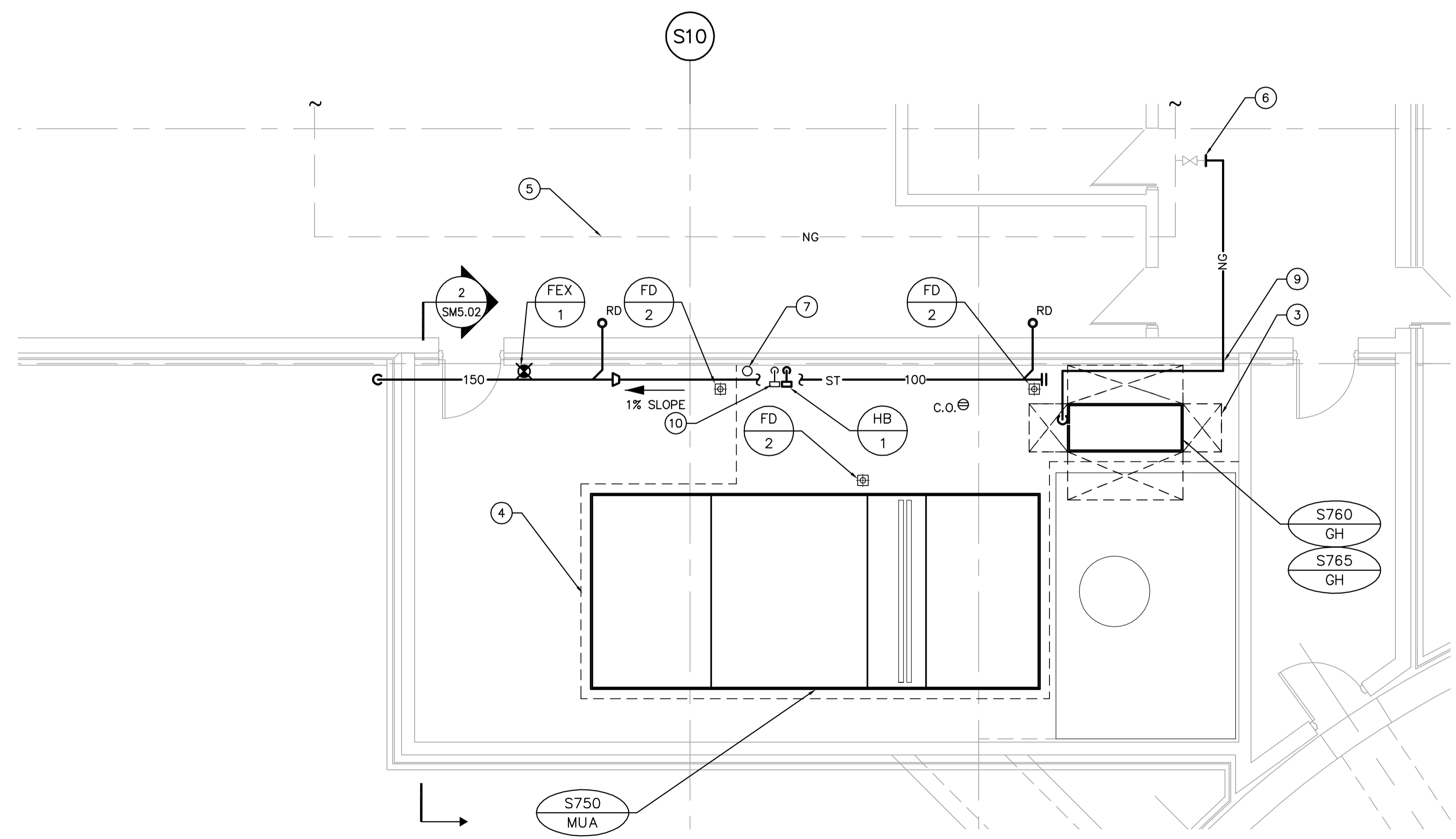
MECHANICAL ROOM - PLUMBING PLAN SCALE: 1:50
