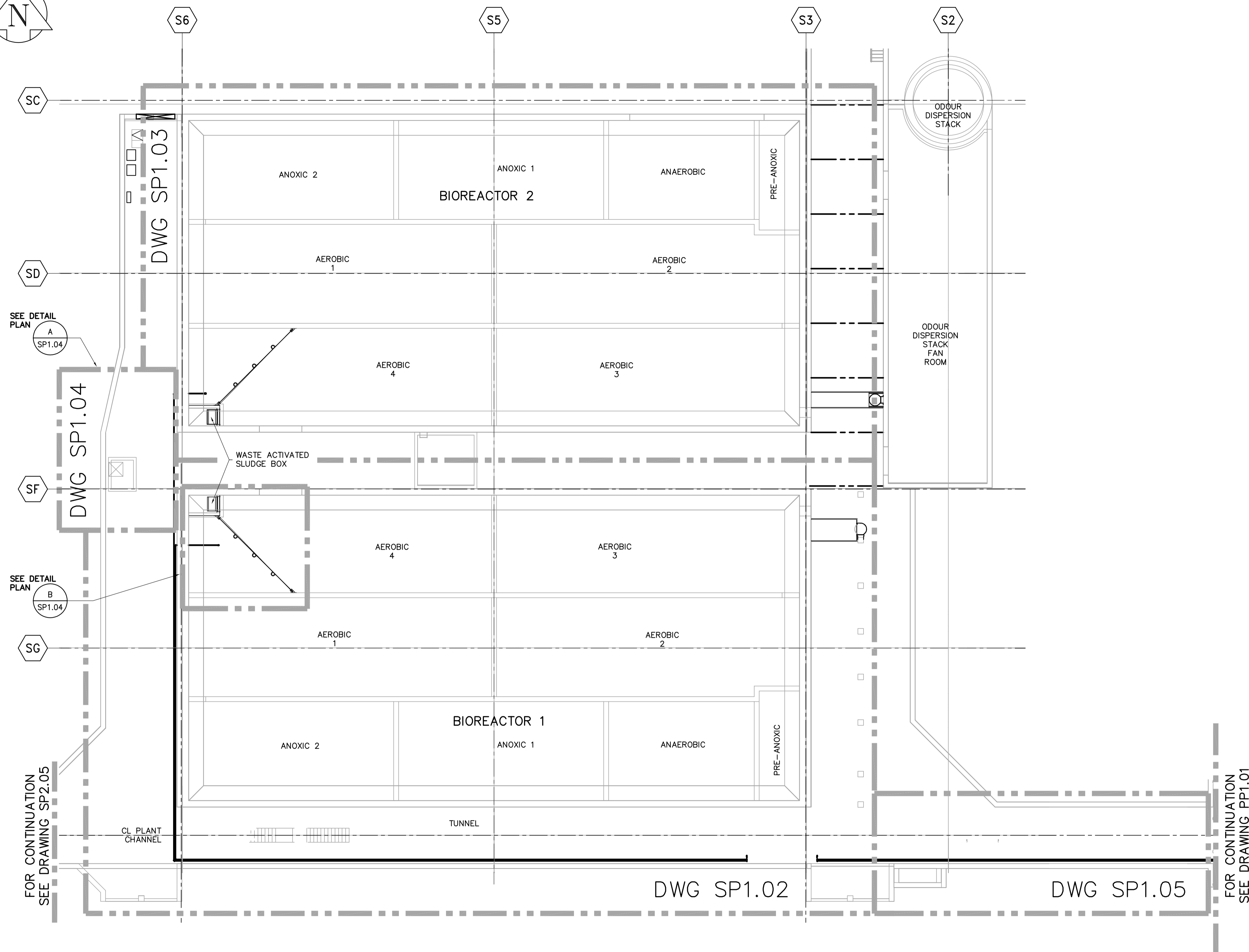
⊙ BIOREACTOR 1 AND 2 - PLAN 1:150
