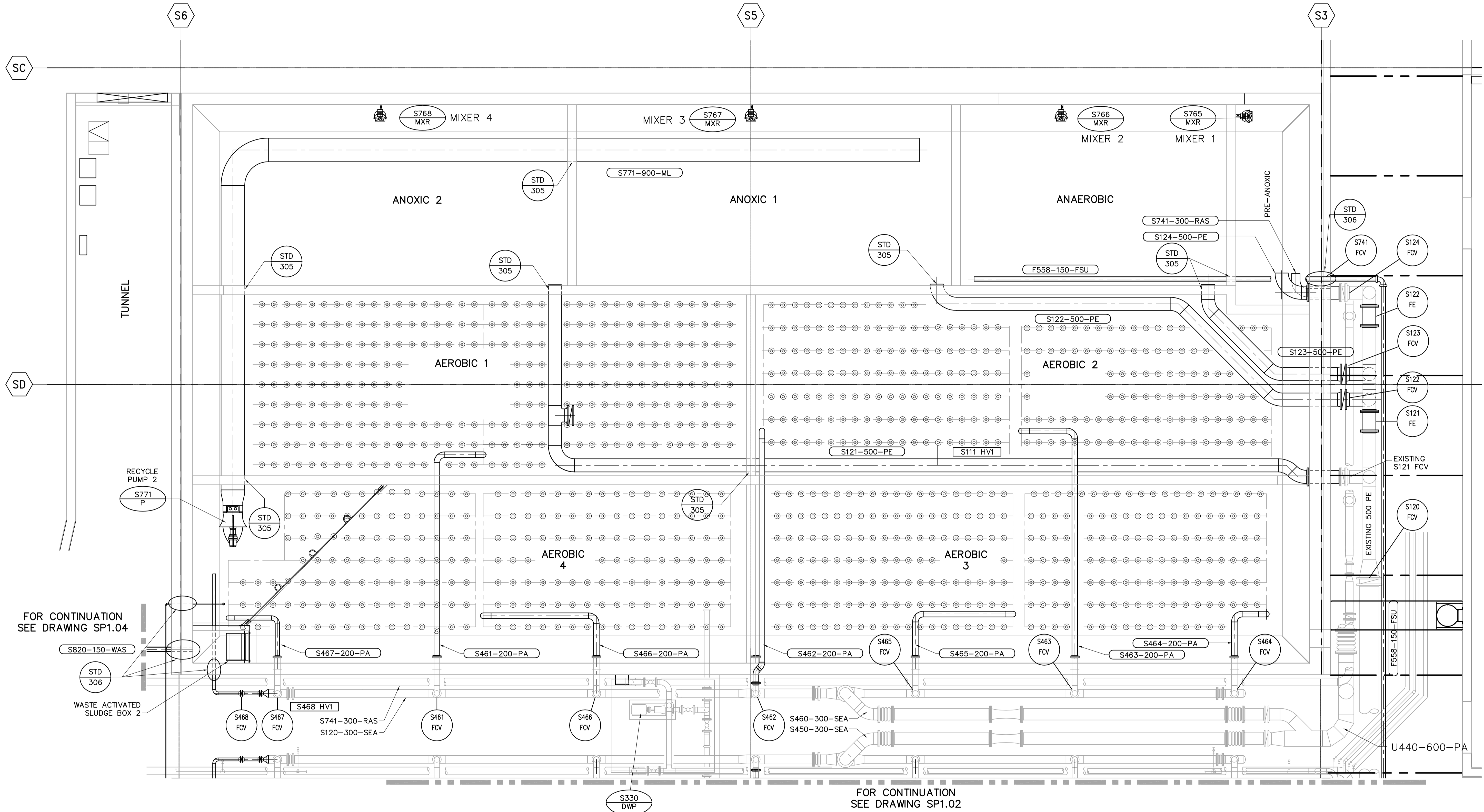
BIOREACTOR 2 - PLAN 1:75
