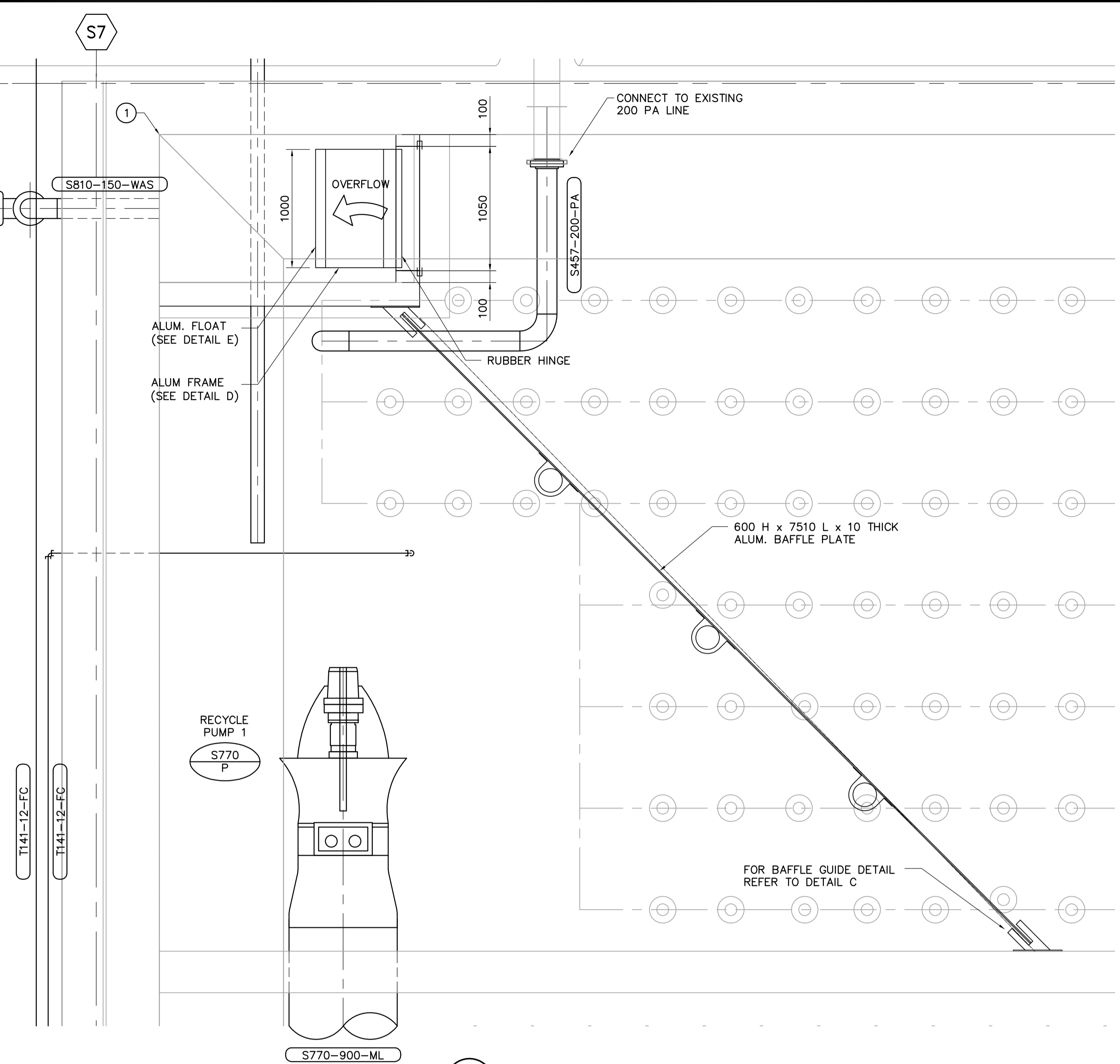
B WAS BOX AND BAFFLE DETAIL SP1.01 1:25
