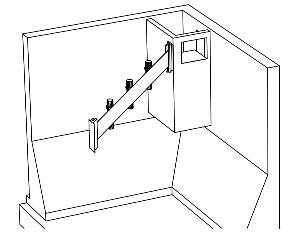
F WAS AREA ISOMETRIC 1:25
