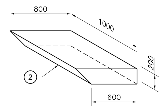
E WAS BOX FLOAT DETAIL 1:25
