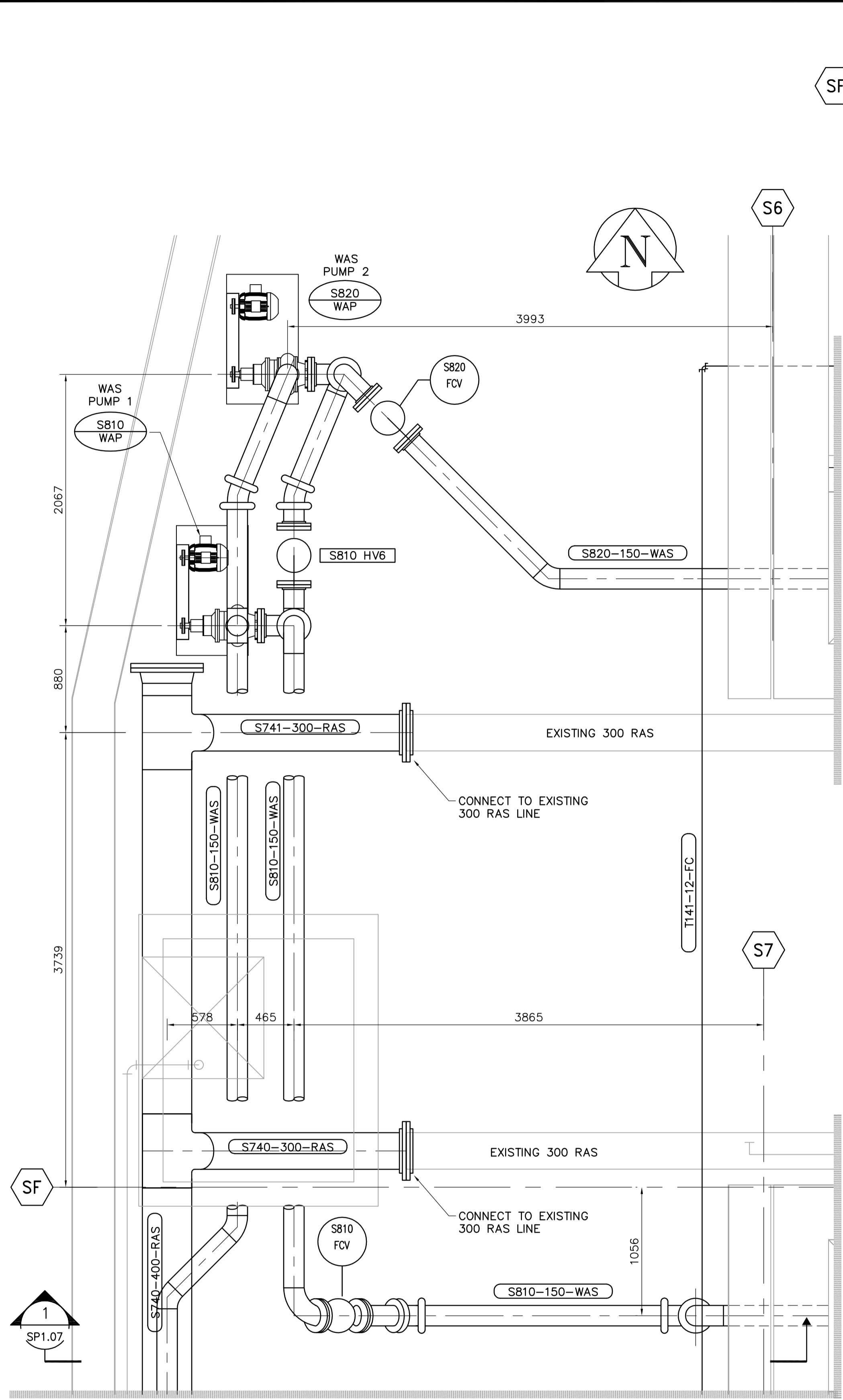
A DETAIL PLAN - WAS PUMPING SP1.01 1:25
