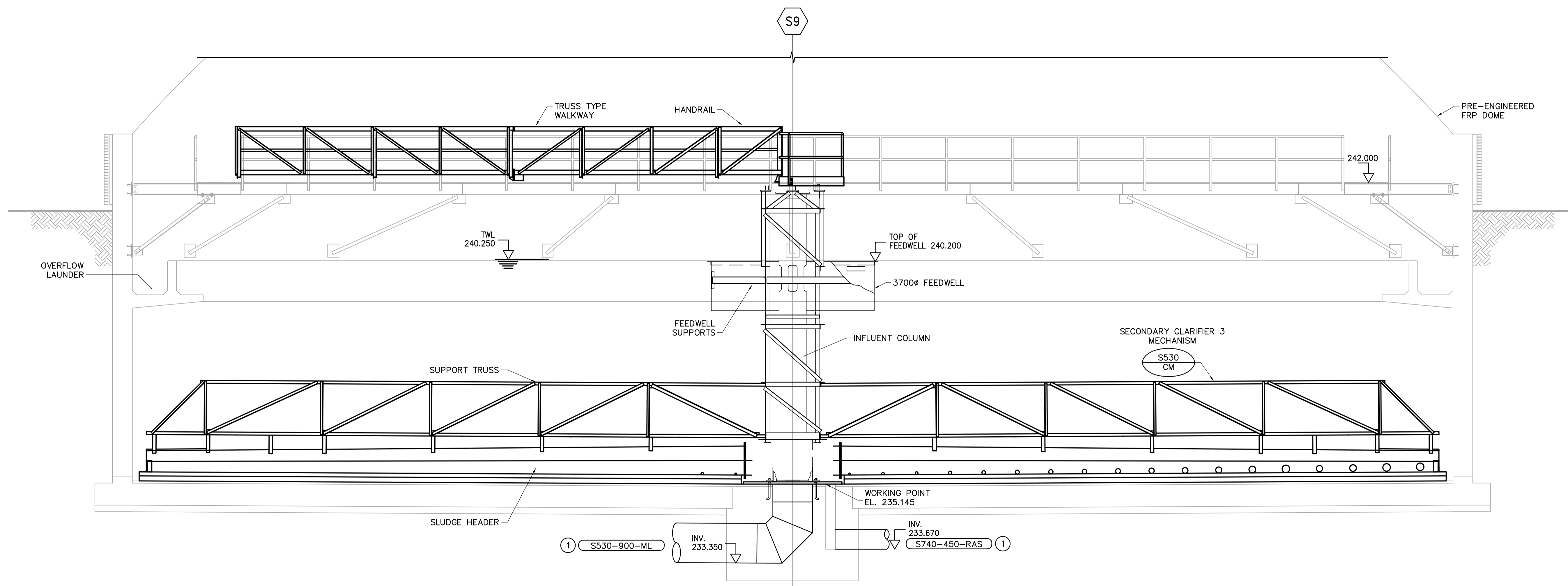
SECTION SP2.01 1:50
