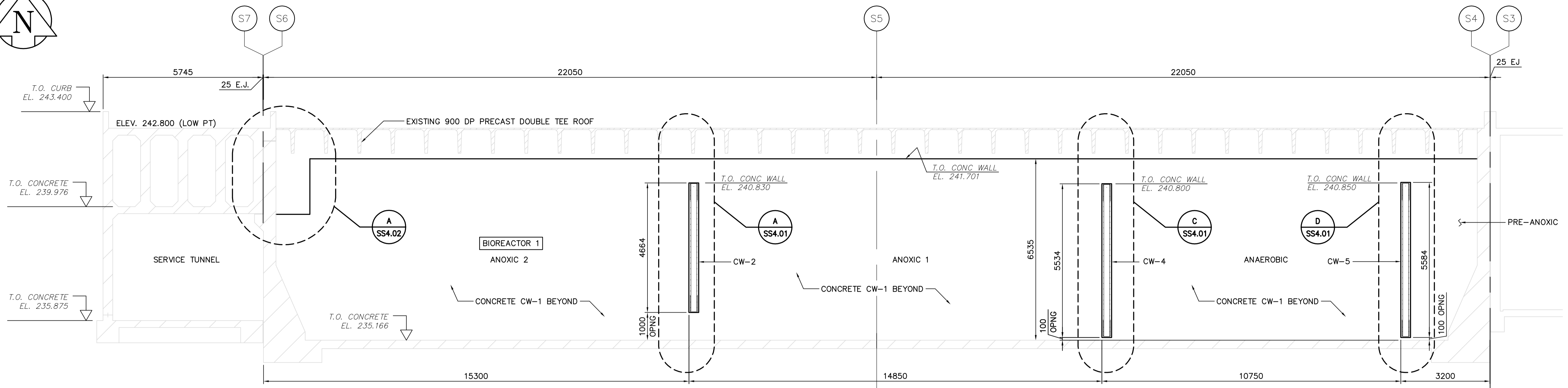
1 SECTION SS2.01 SCALE 1:75
