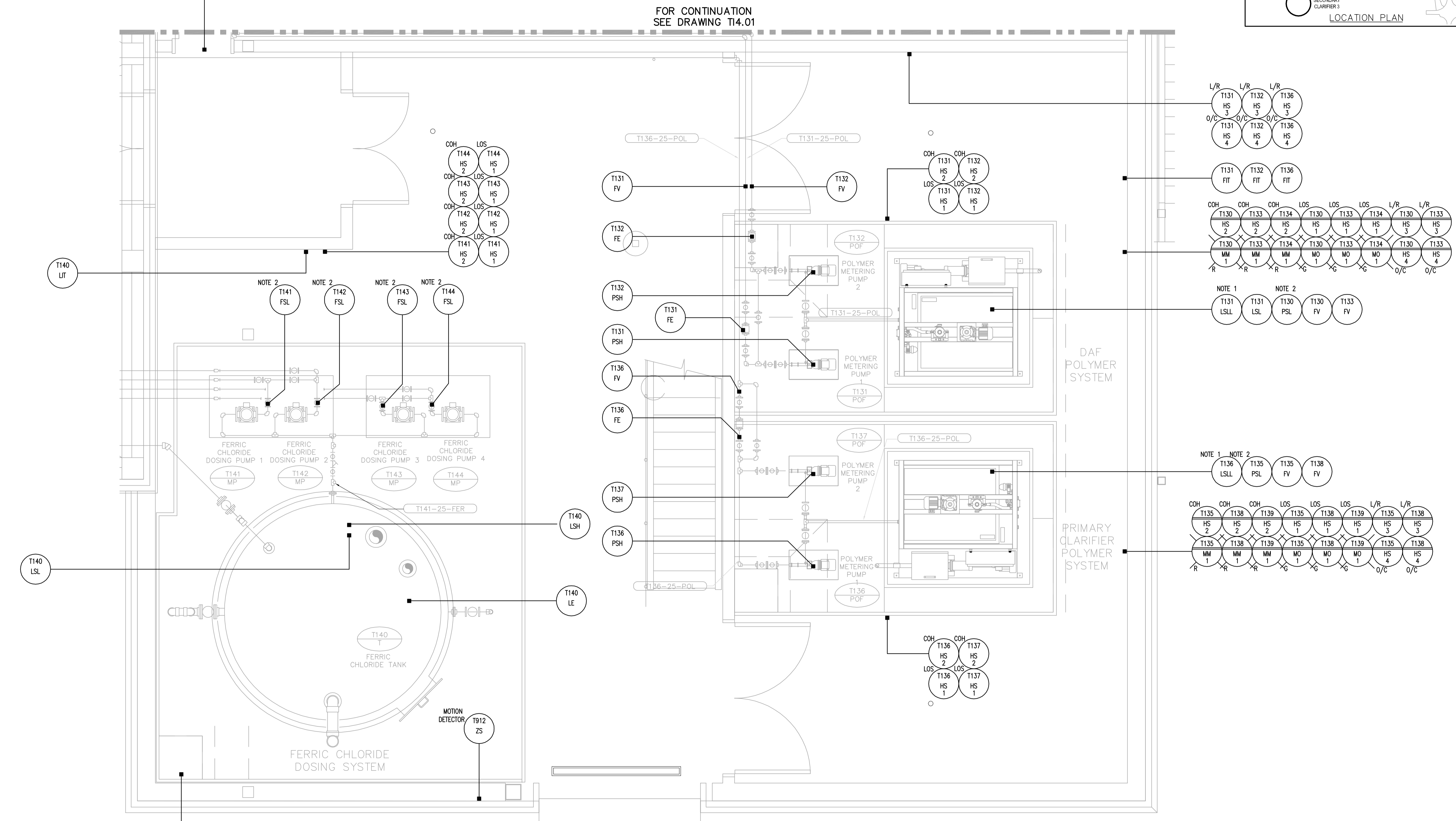
LOCATION PLAN - POLYMER / FERRIC ROOMS 1:50
