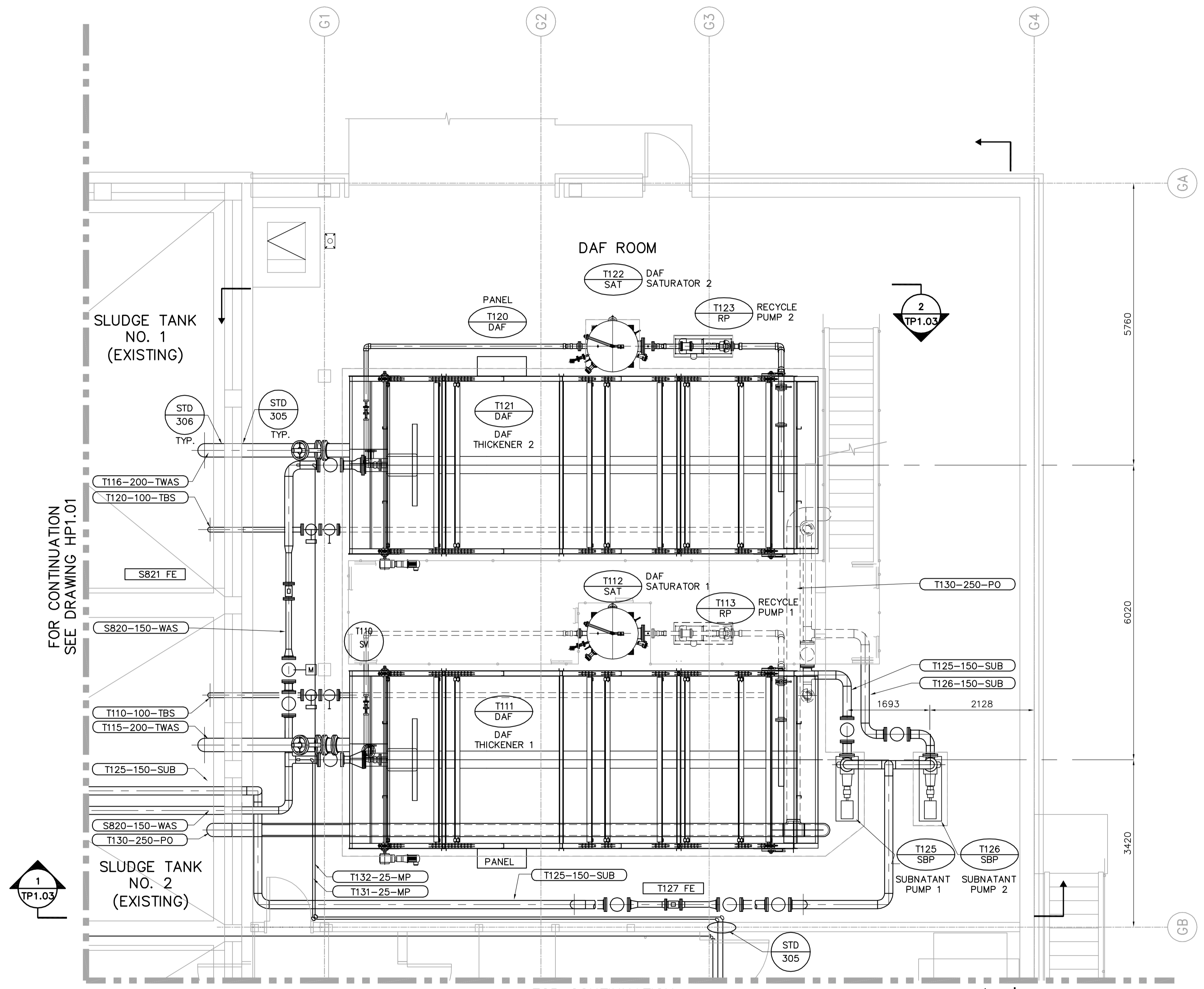
PLAN - DAF BUILDING 1:50
