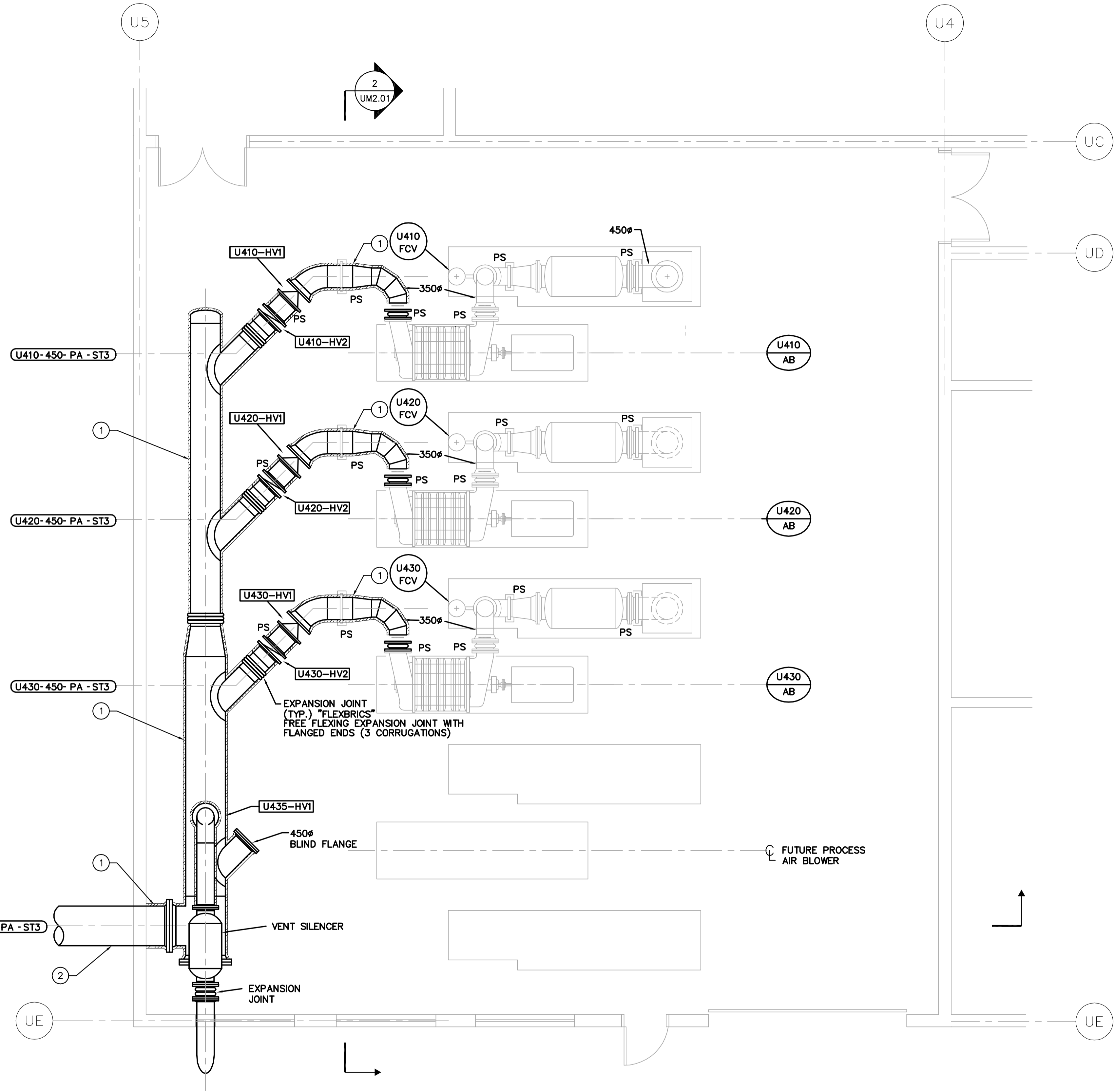
BLOWER ROOM – PIPING INSULATION PLAN SCALE: 1:50
