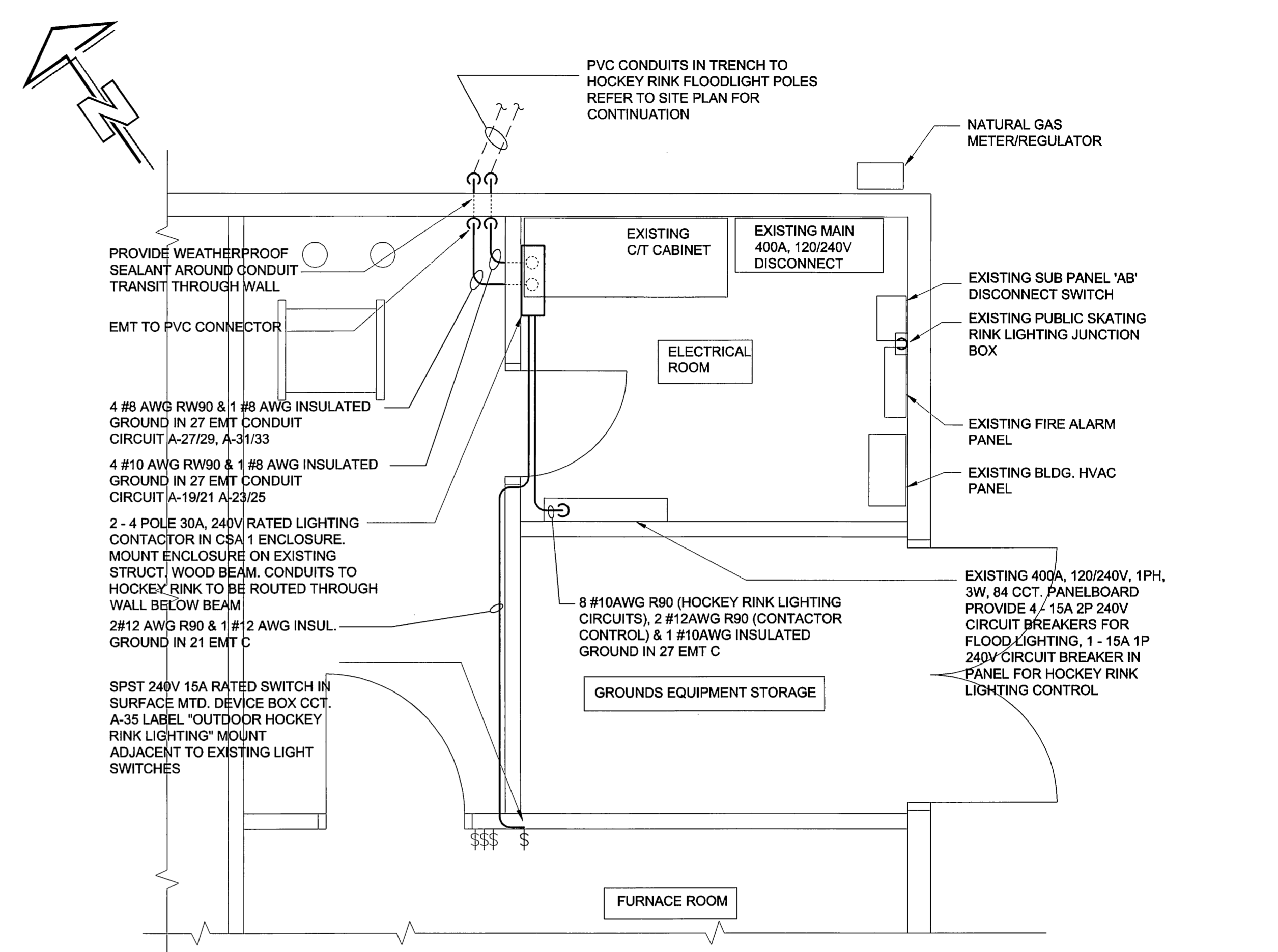
PARTIAL FLOOR PLAN
