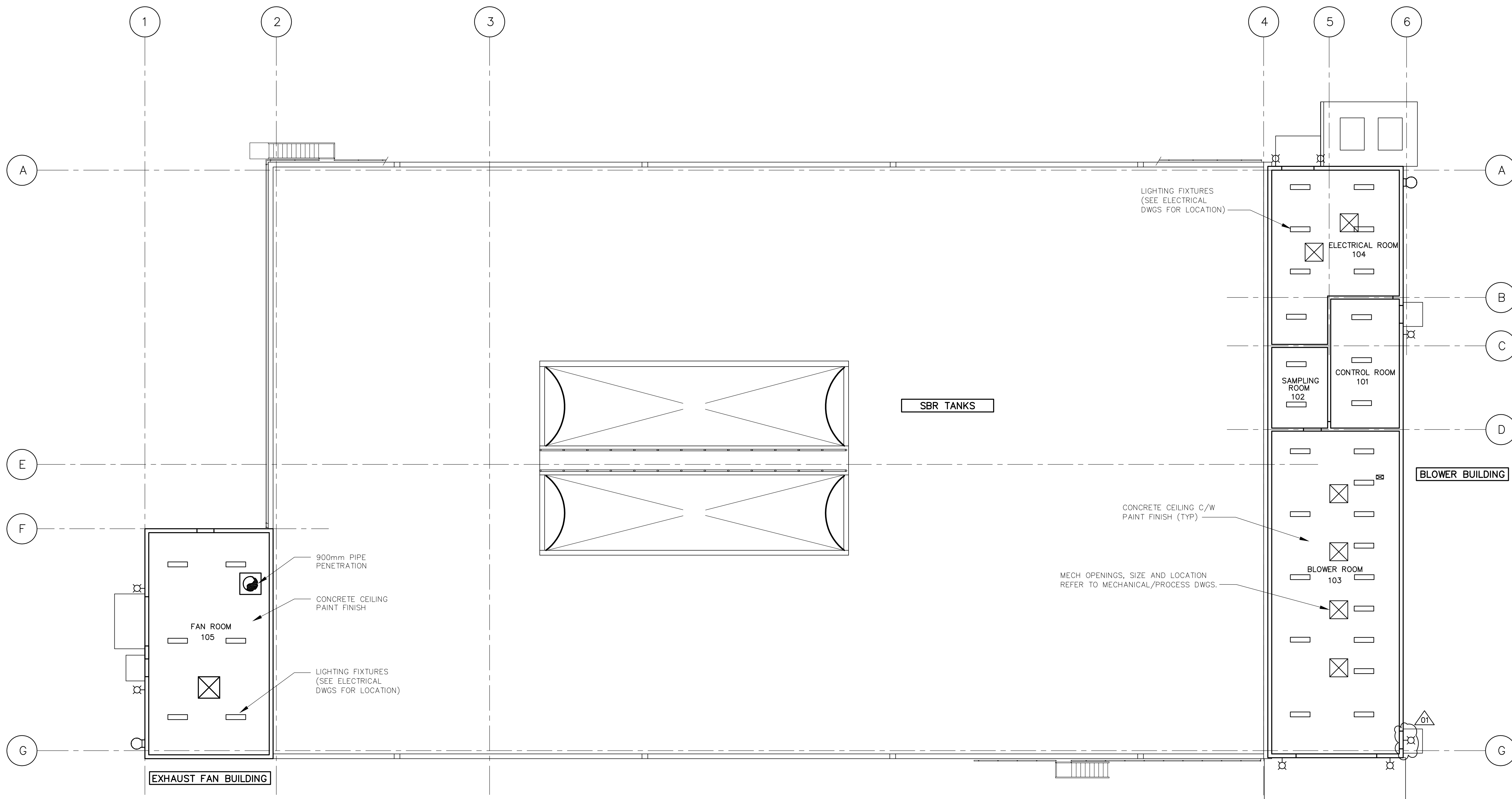
1 REFLECTED CEILING PLAN A1.04 1:125
