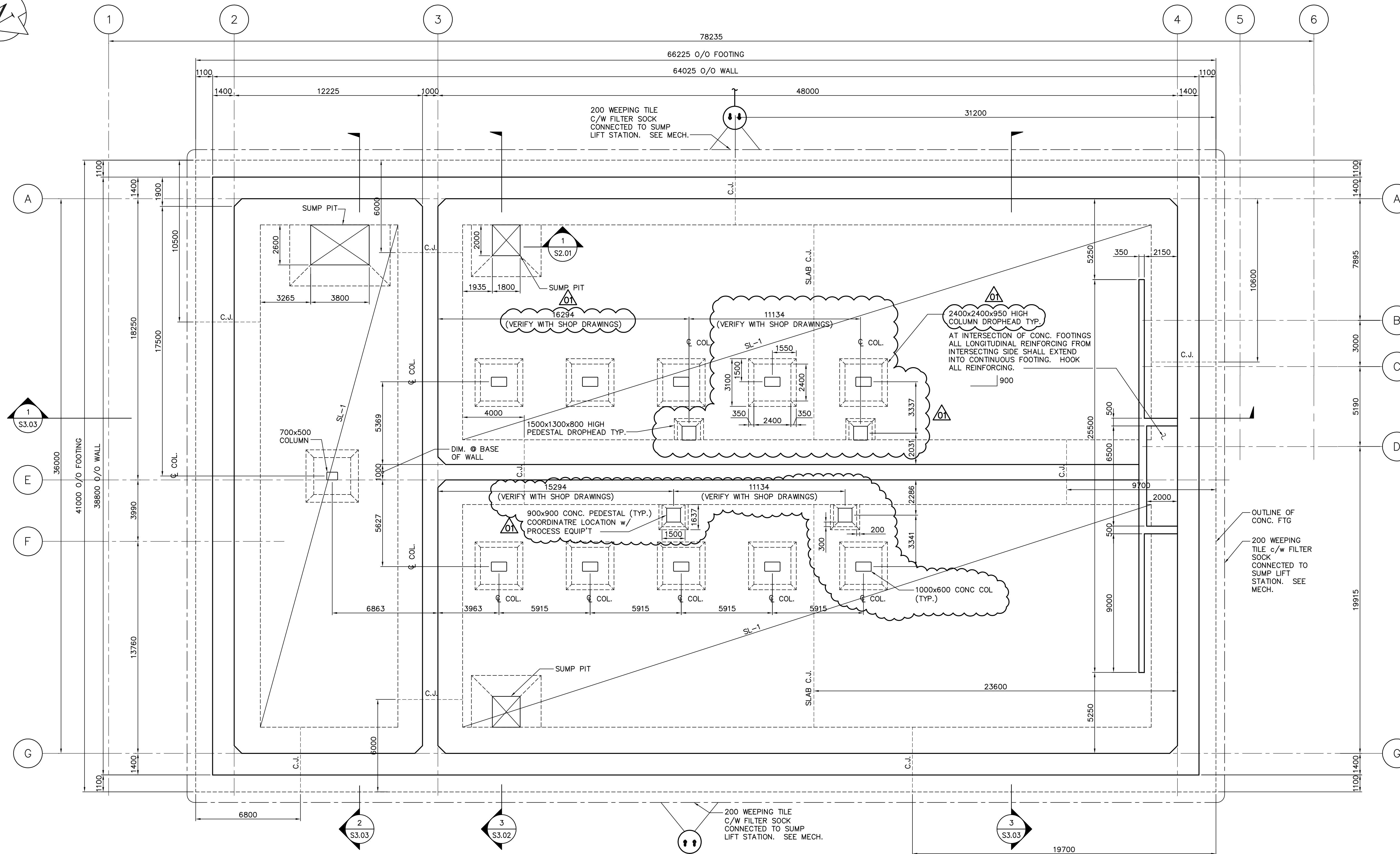
B FLOOR PLAN @ ELEV. 223.910 SCALE 1:125
