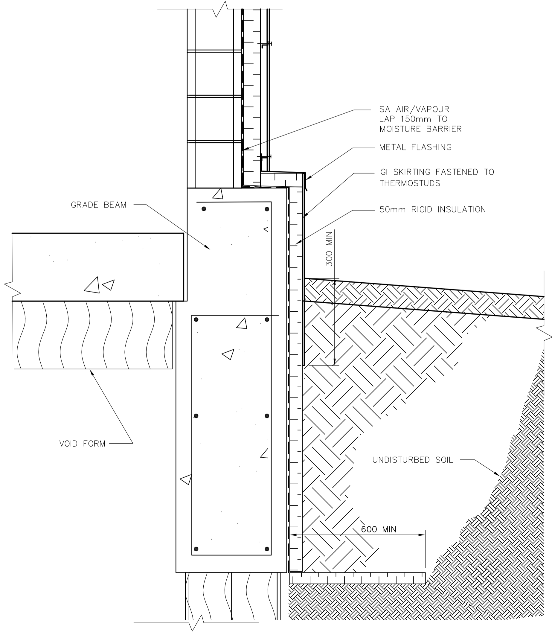
3 WALL SECTION DETAIL A3.01 1:10
