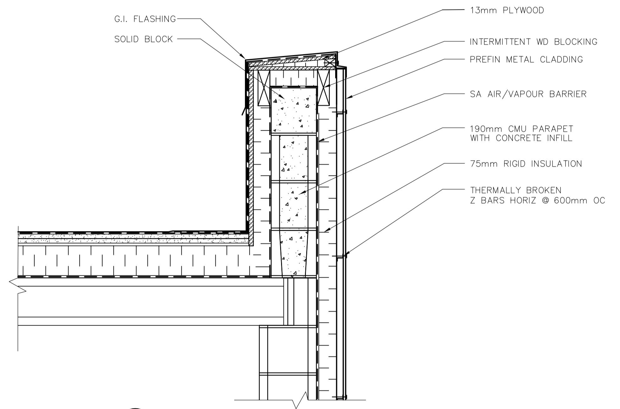
5 PARAPET DETAIL (TYP) A3.02 1:10
