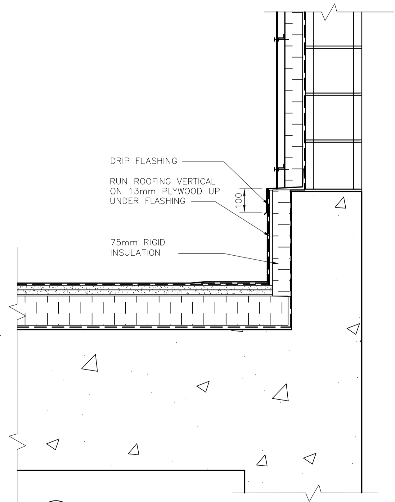
2 ROOF TO WALL SECTION A3.01 1:125
