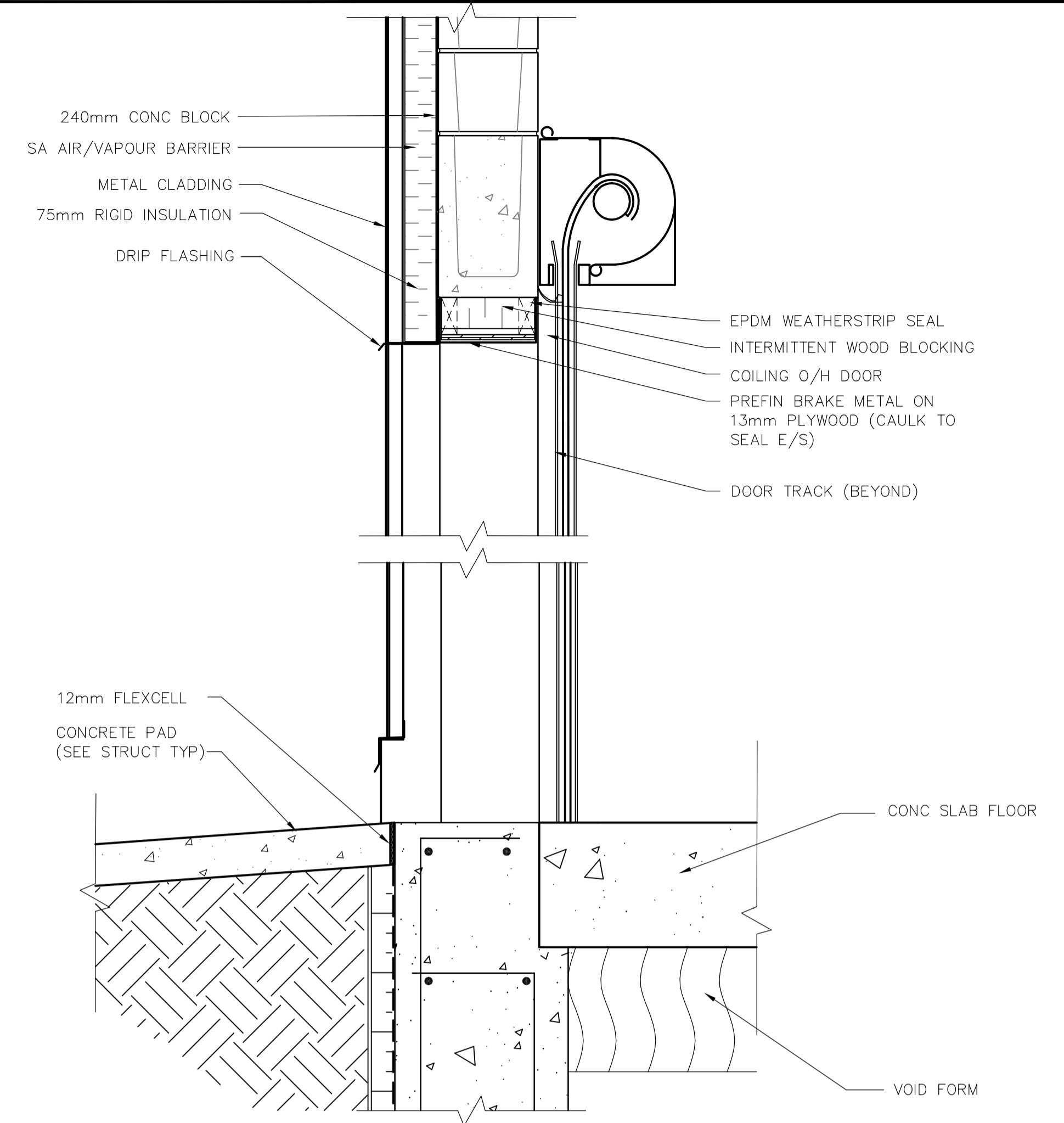
4 OVERHEAD COILING DOOR SECTION DETAIL A3.02 1:10
