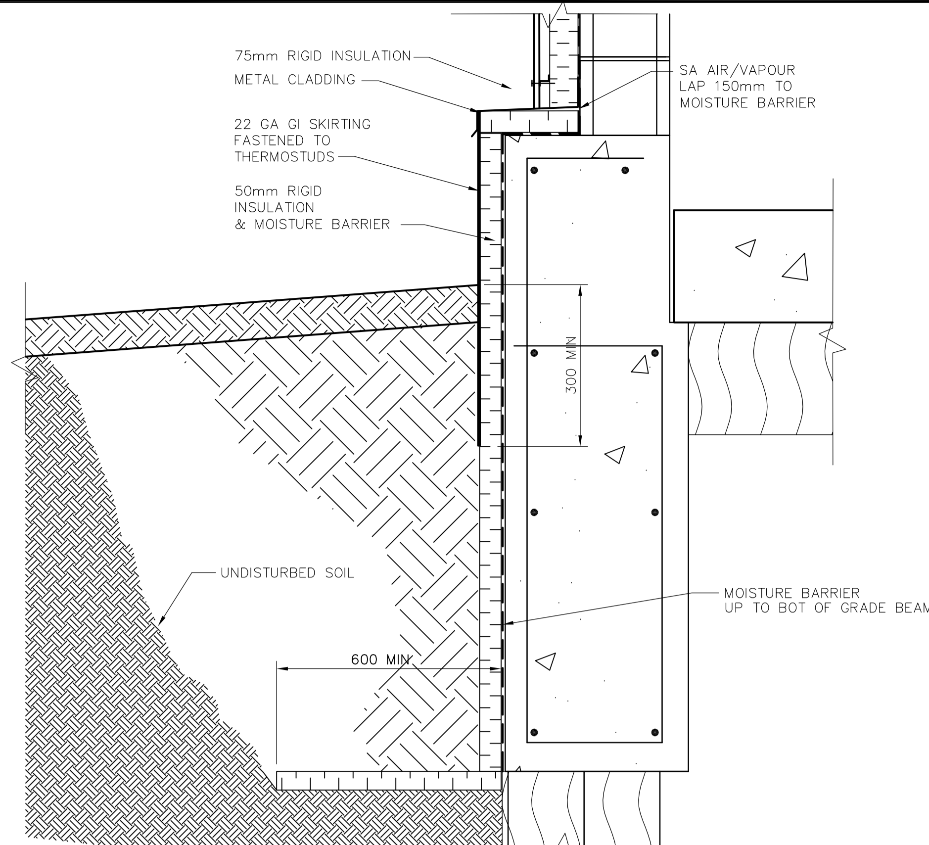
1 FOUNDATION WALL SECTION DETAIL A3.01 1:10
