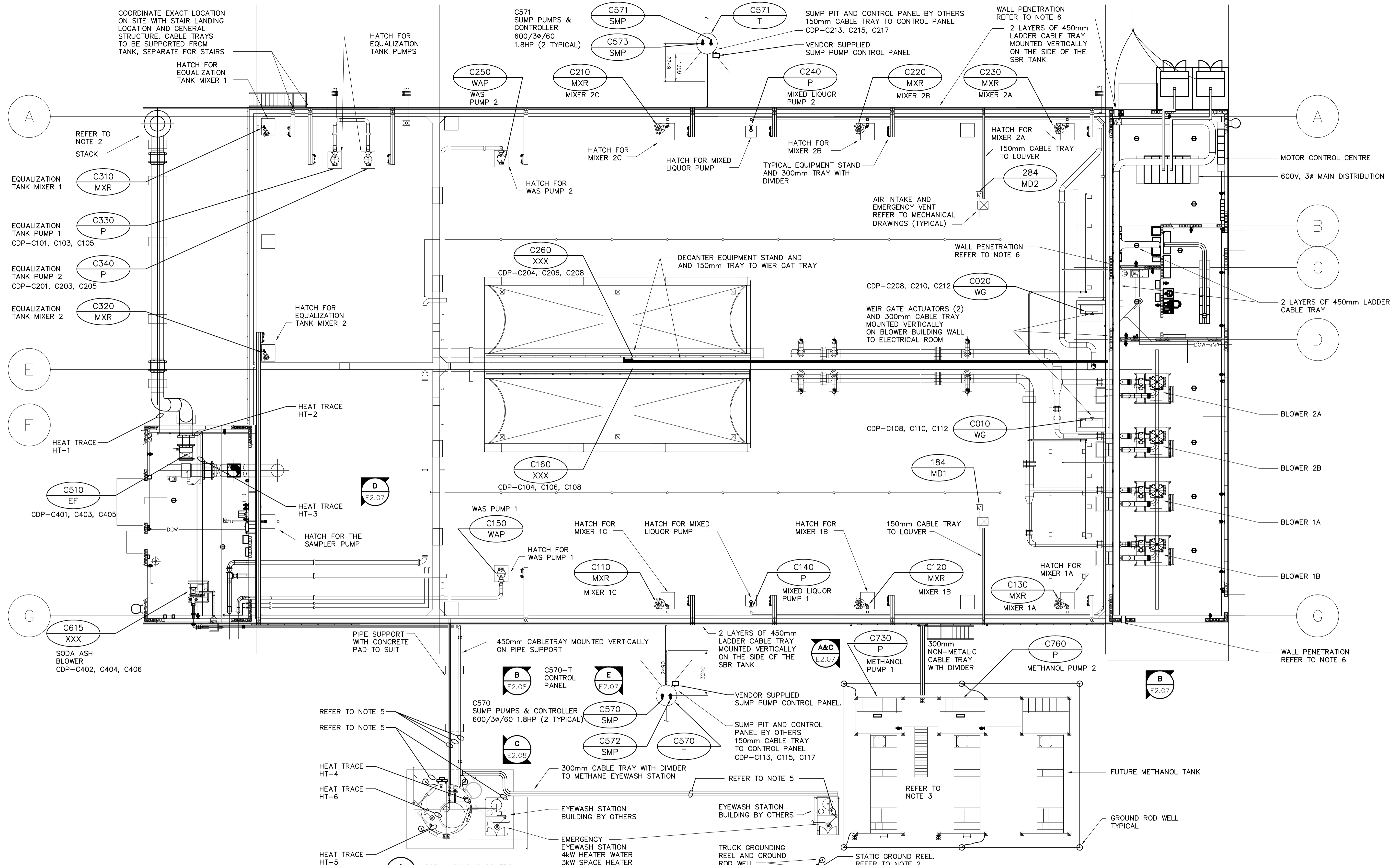
1 E2.05 DETAIL - SBR BASIN AND EQUALIZATION TANKS PLAN SCALE: N.T.S.
