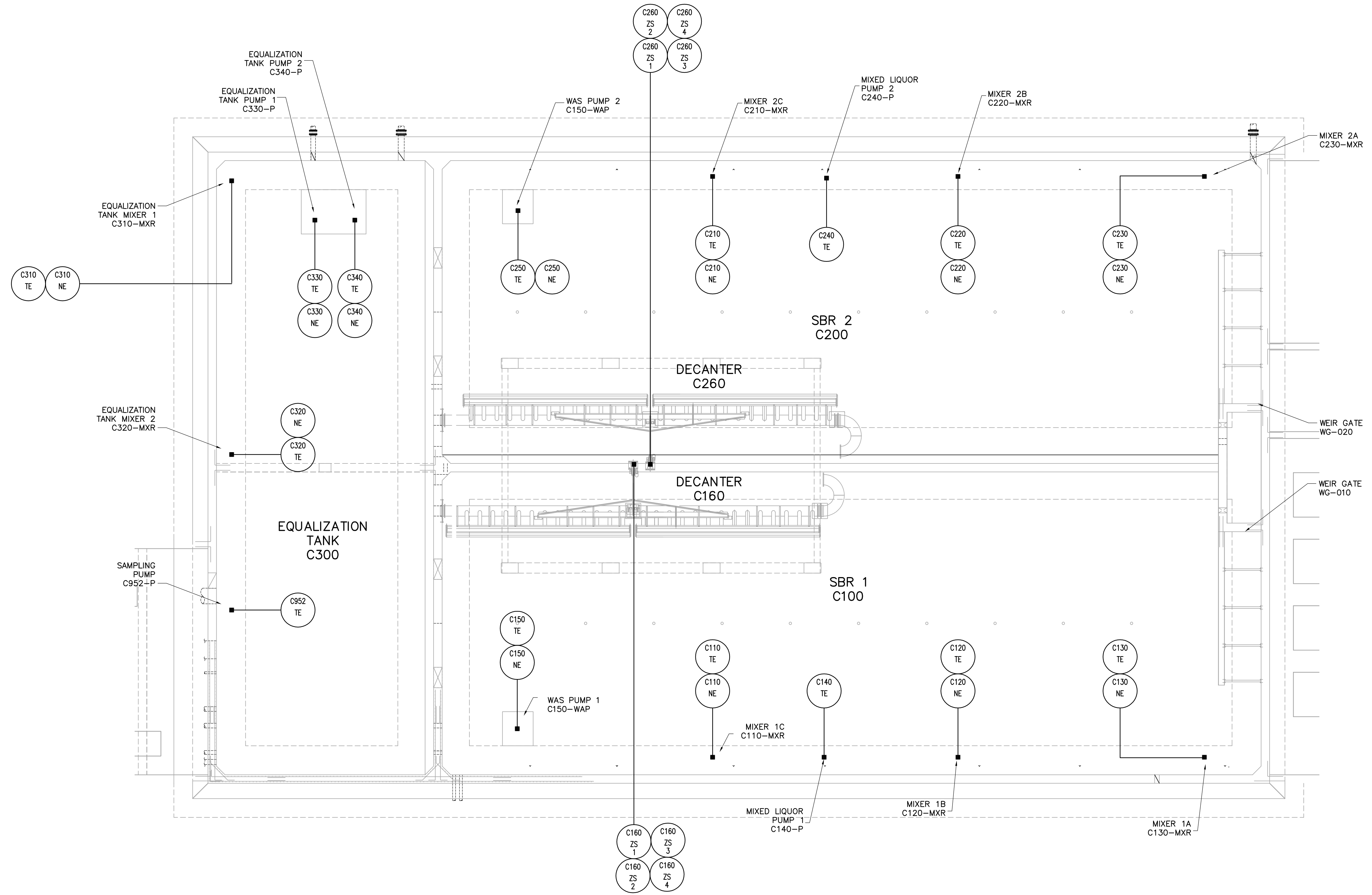
1 LOWER LEVEL - PROCESS TANKS INSTRUMENT PLAN SCALE 1:125
