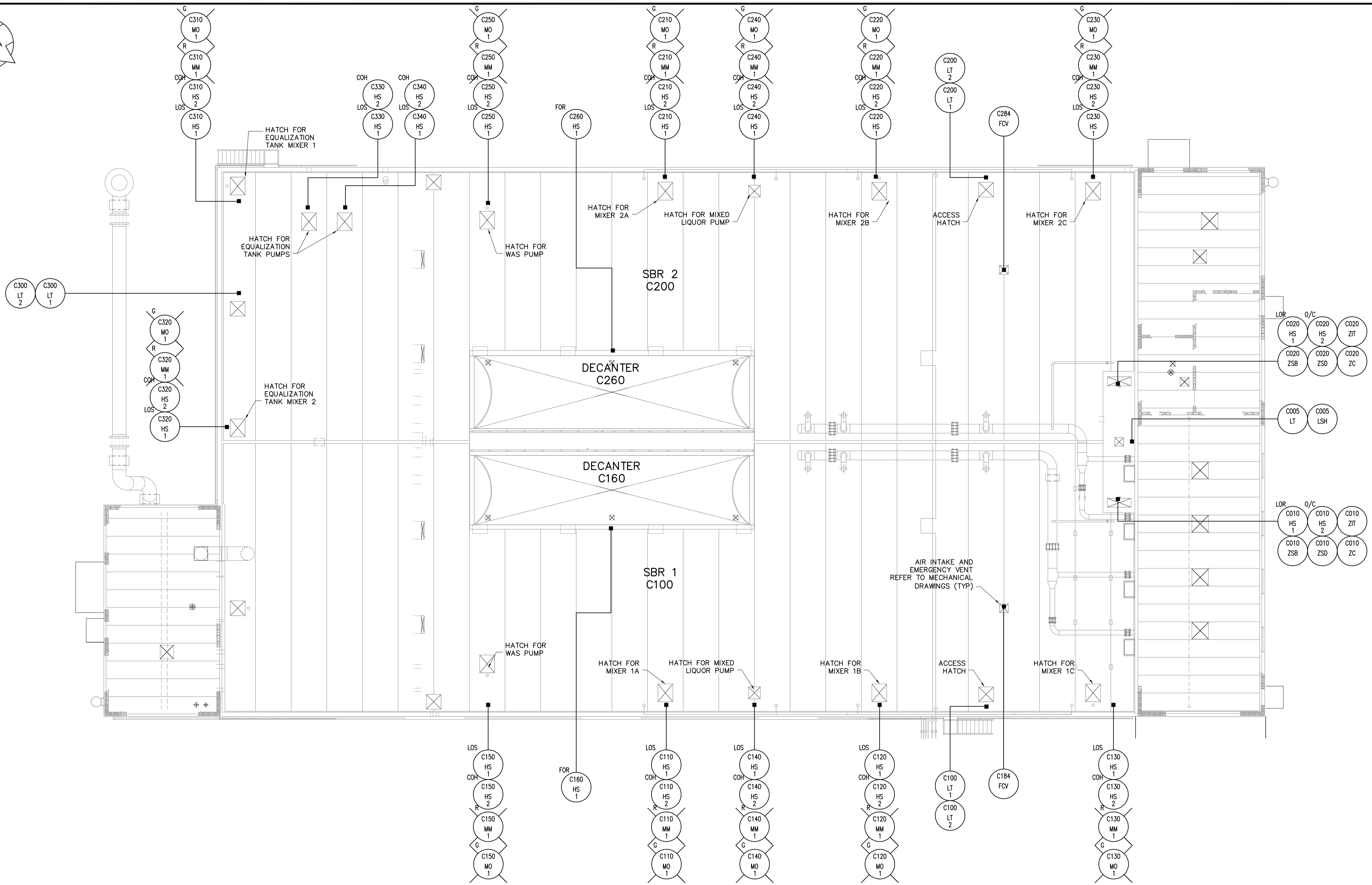
1 UPPER LEVEL PLAN - PROCESS TANKS INSTRUMENT PLAN SCALE 1:125
