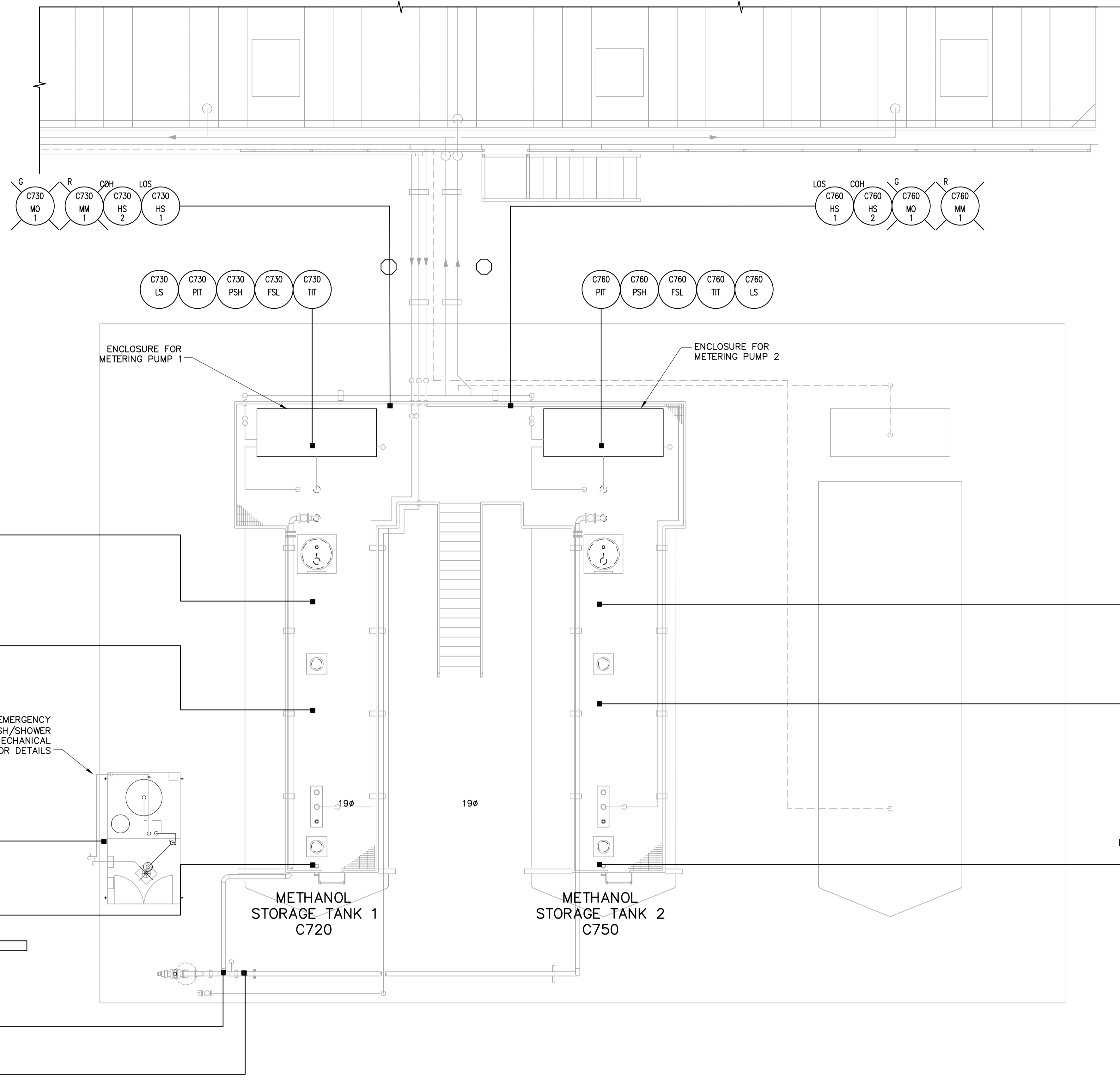
1 METHANOL DOSING TANKS INSTRUMENT PLAN SCALE 1:50
