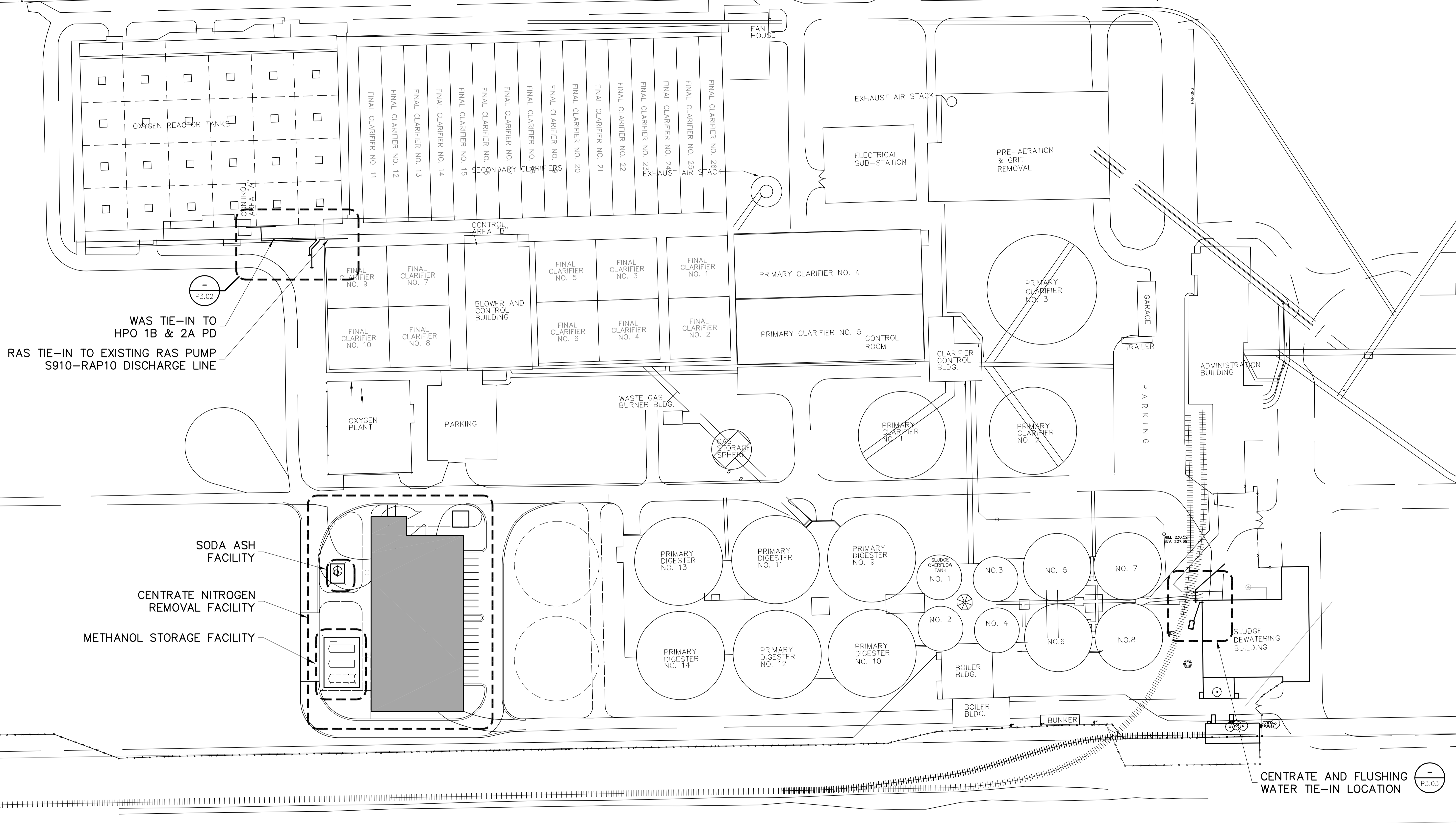
LOCATION PLAN SCALE 1:1000
