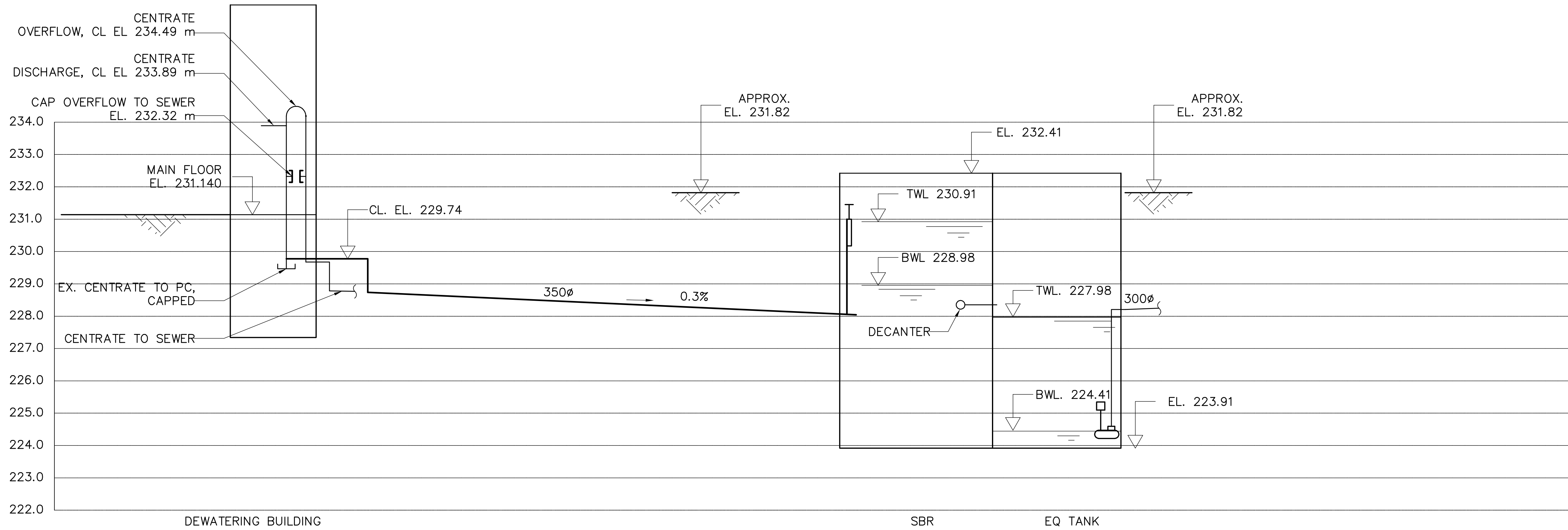
A CENTRATE AND TREATED CENTRATE TRANSFER SCALE 1:100
