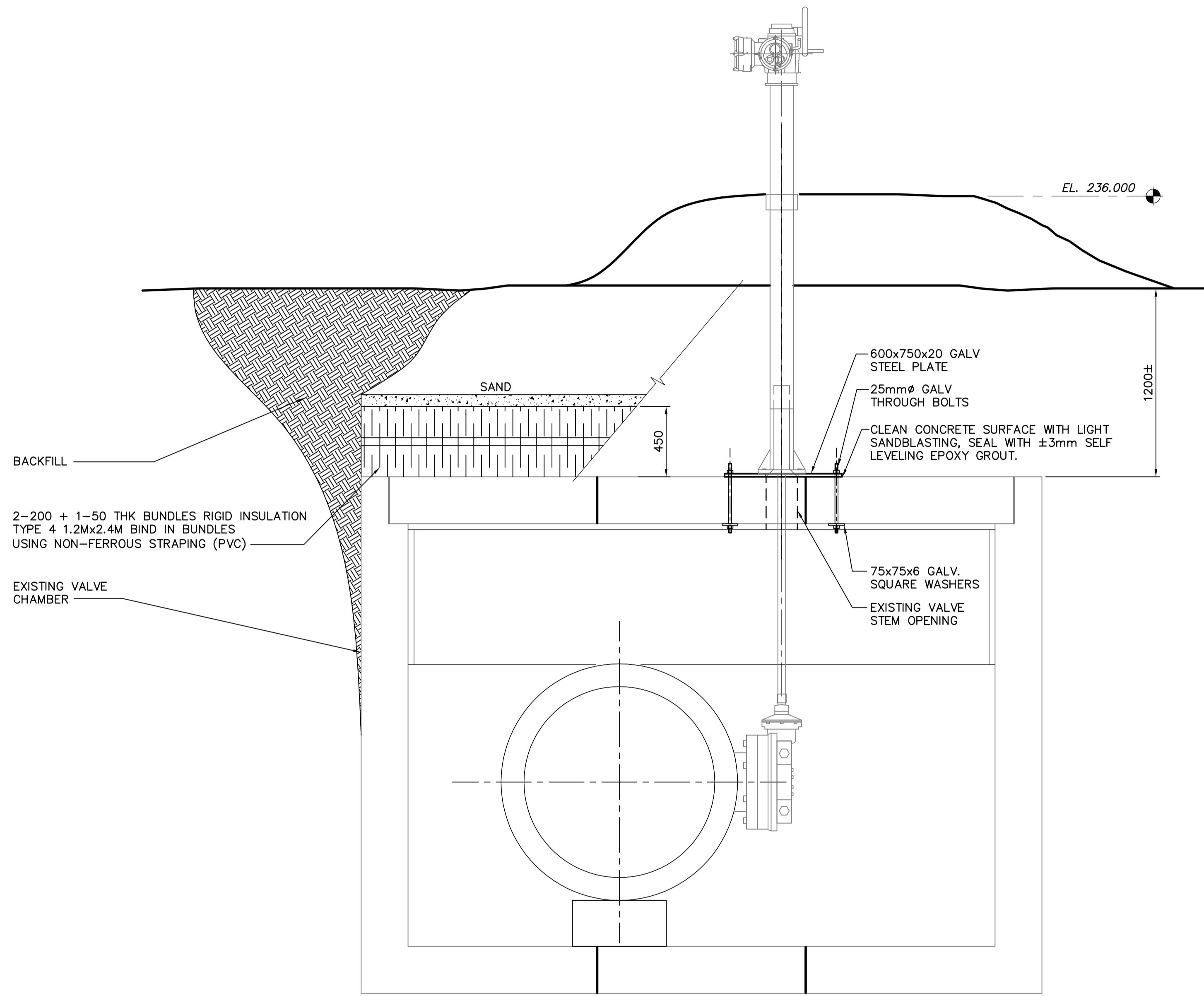
SECTION 1:20
