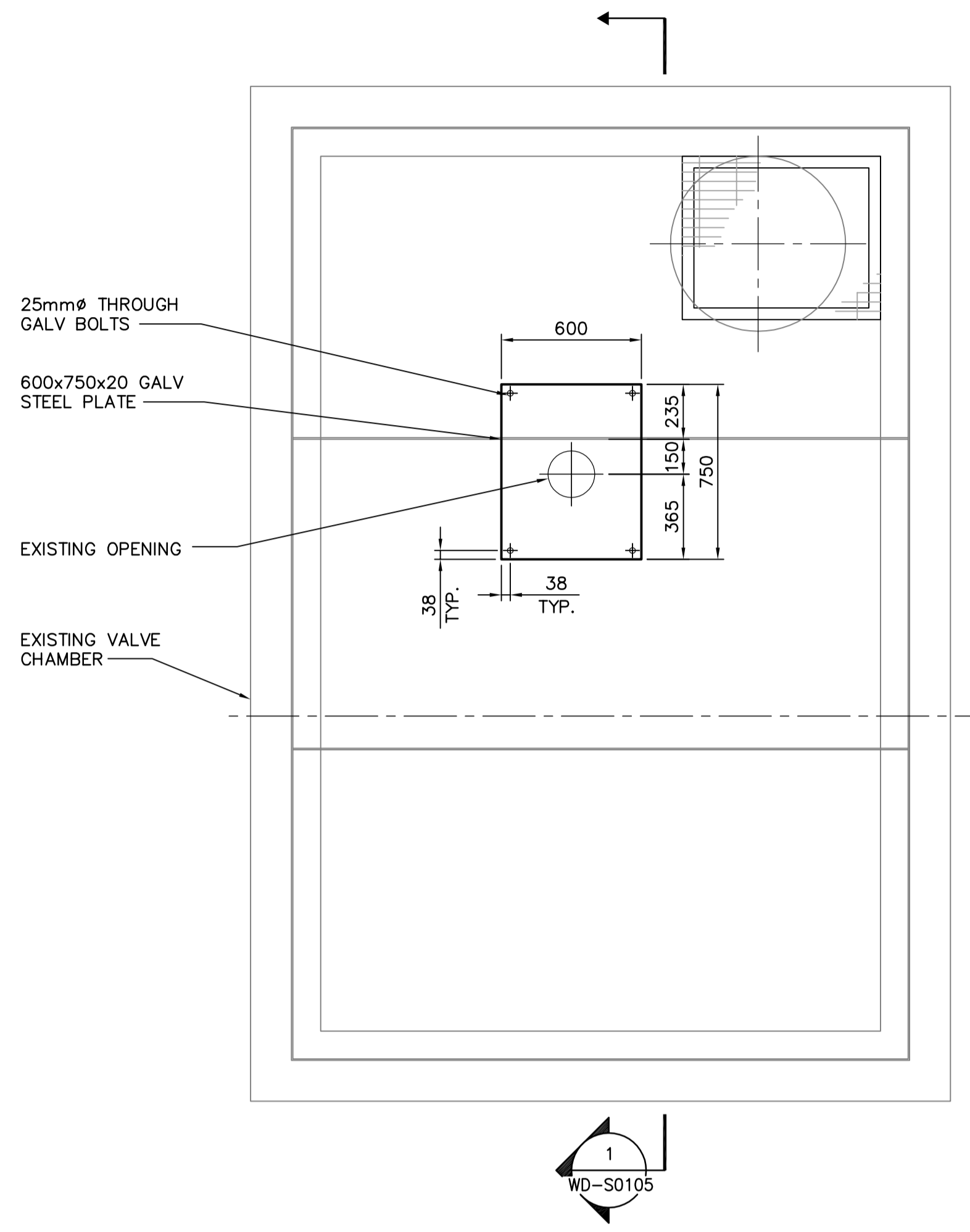
DRV 305 VALVE CHAMBER ROOF PLAN VIEW 1:20
