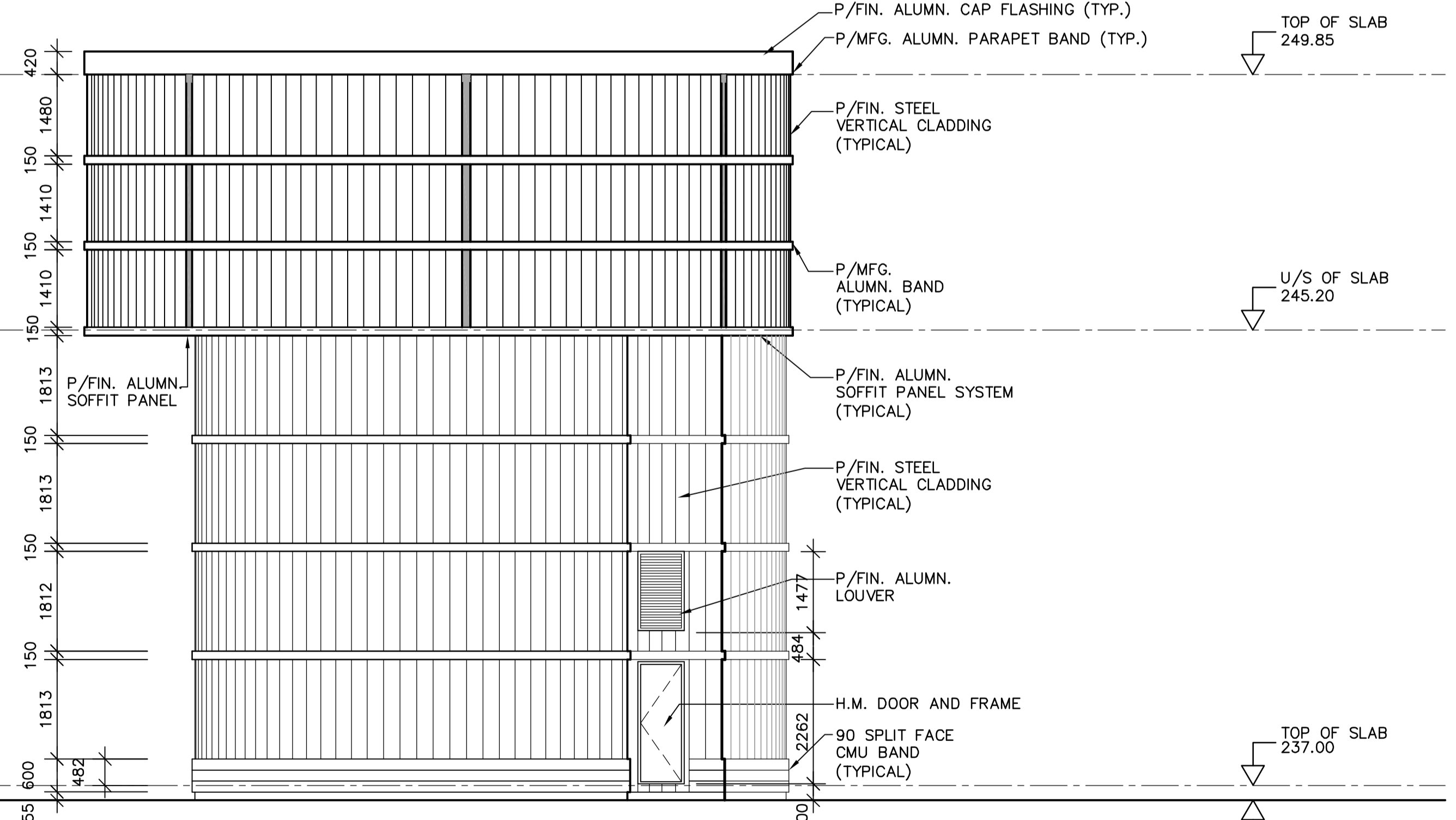
2-EAST ELEVATION SCALE 1:75
