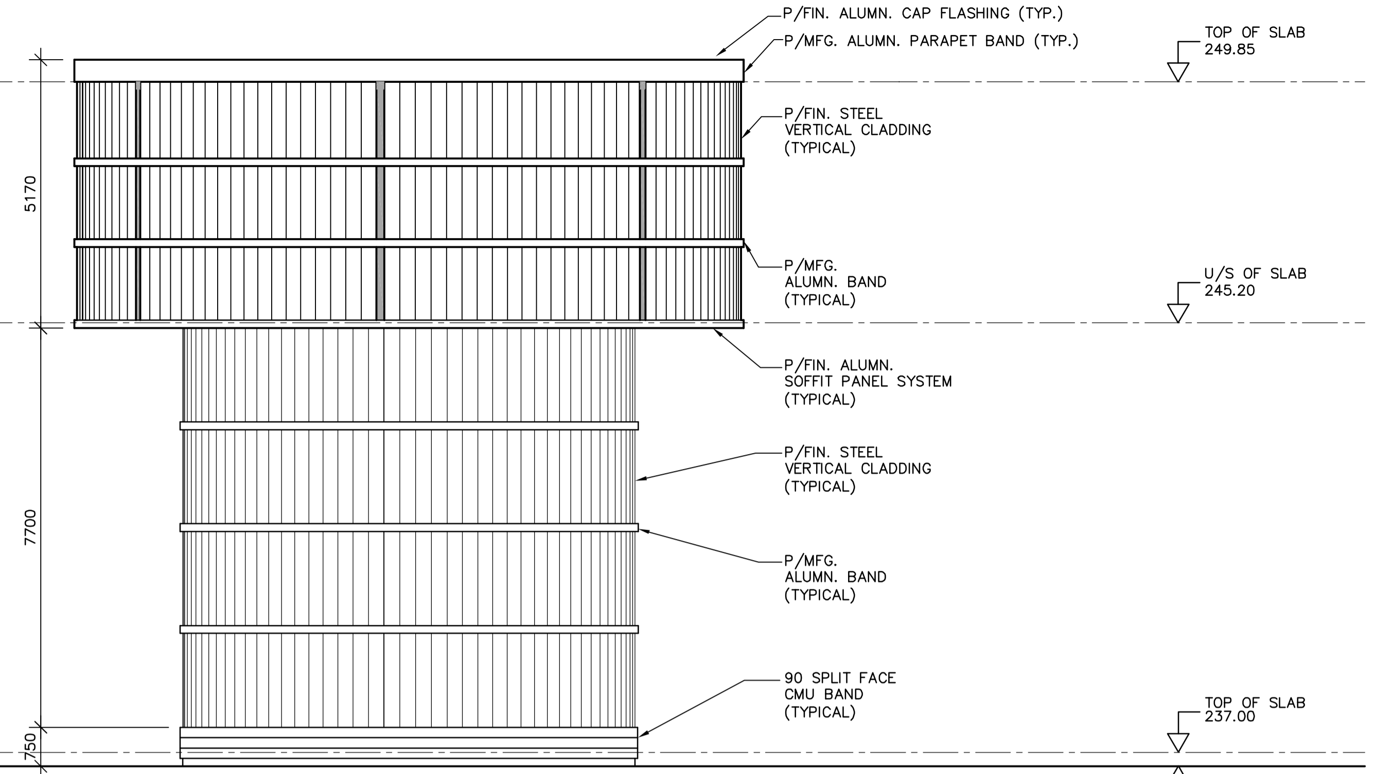
3-SOUTH ELEVATION SCALE 1:75
