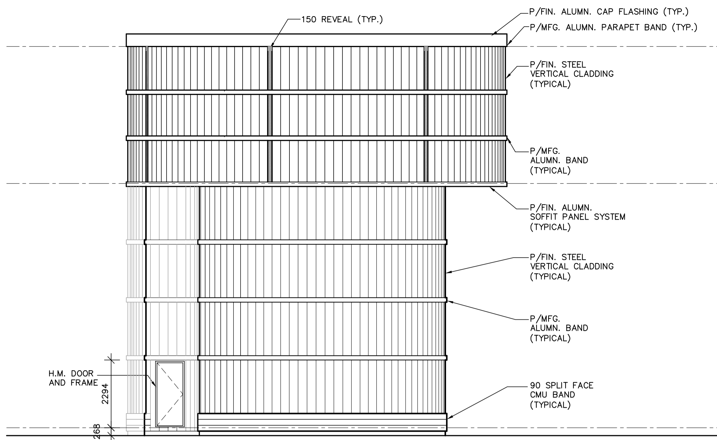
4-WEST ELEVATION SCALE 1:75
