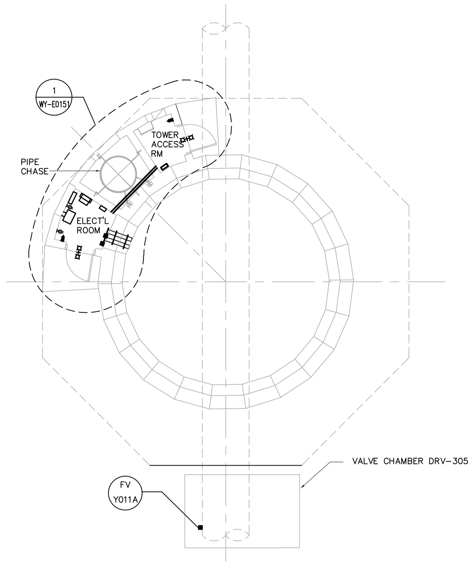
MAIN ENTRY PLAN @ EL. 236.500
