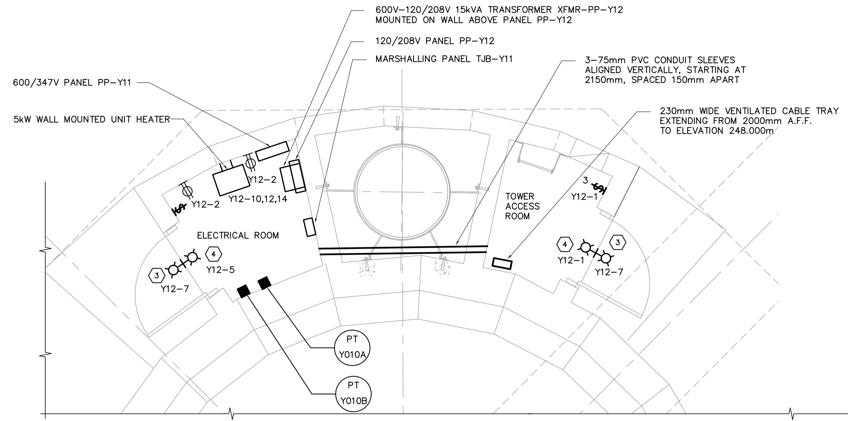
PARTIAL PLAN @ MAIN ENTRY
