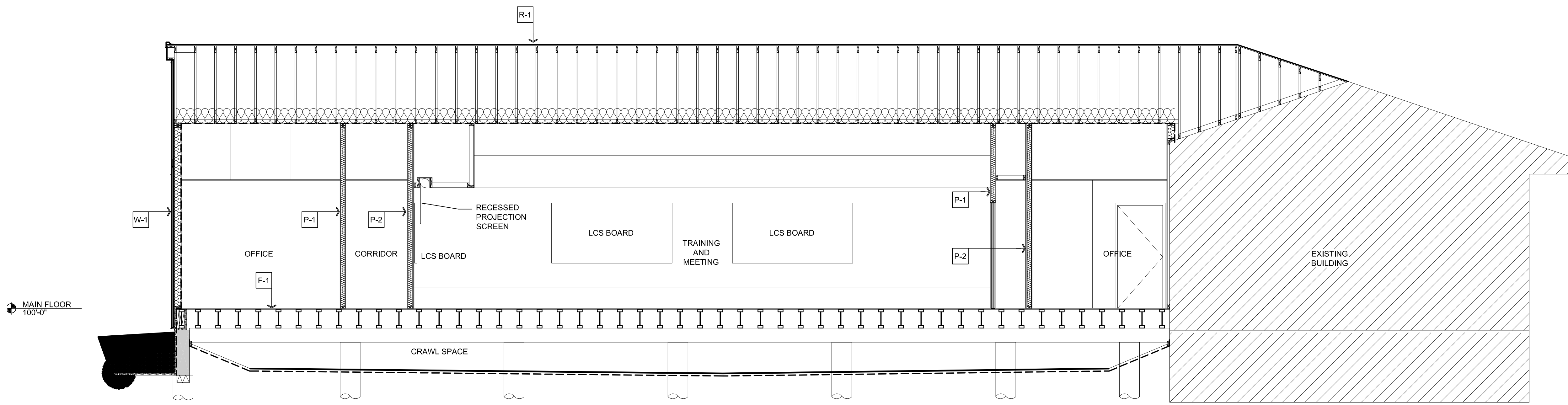
2 BUILDING CROSS SECTION SCALE: 1/4" = 1'-0"
