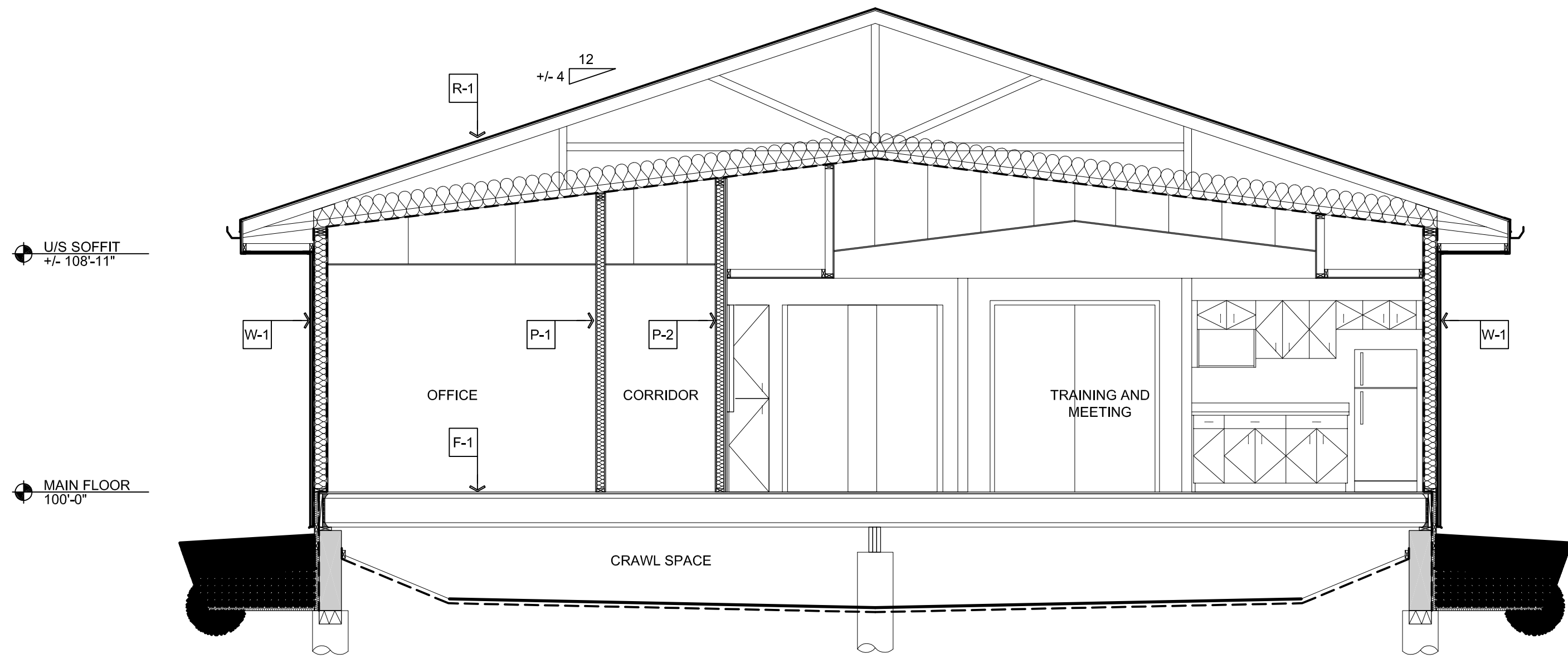
1 BUILDING CROSS SECTION SCALE: 1/4" = 1'-0"
