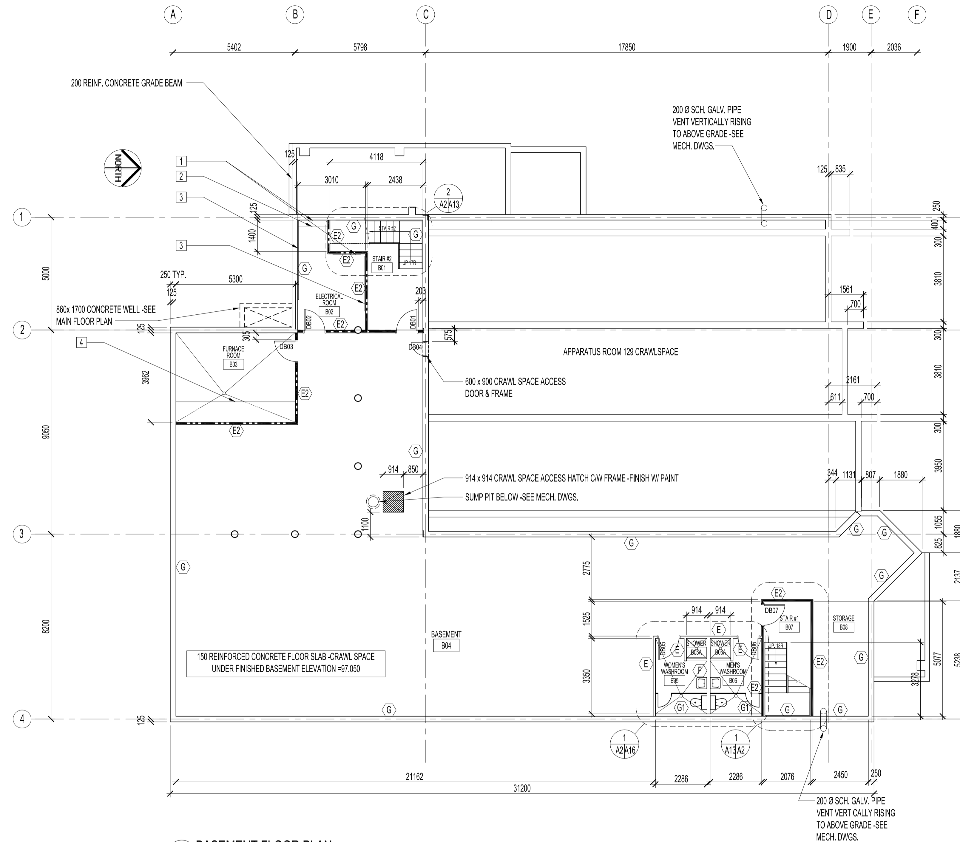
1 BASEMENT FLOOR PLAN A2 SCALE 1:100
