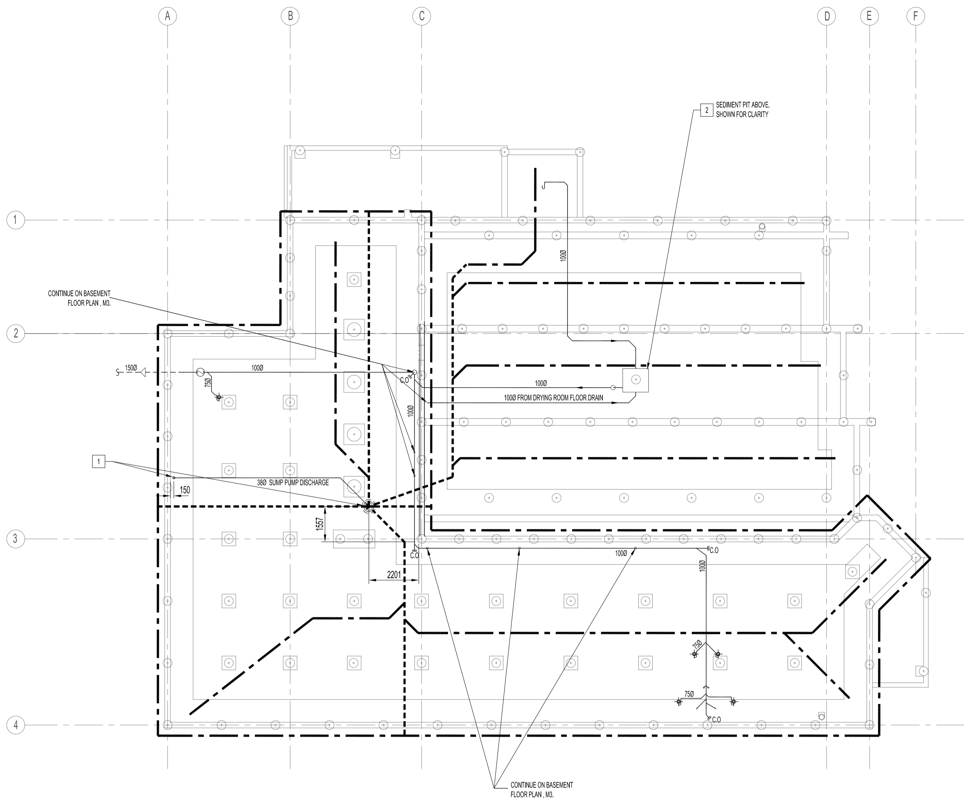
CRAWL SPACE FLOOR PLAN - PLUMBING SCALE: 1:50
