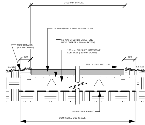
Asphalt Cross-Section Section "A - A" Scale: 1: 25
