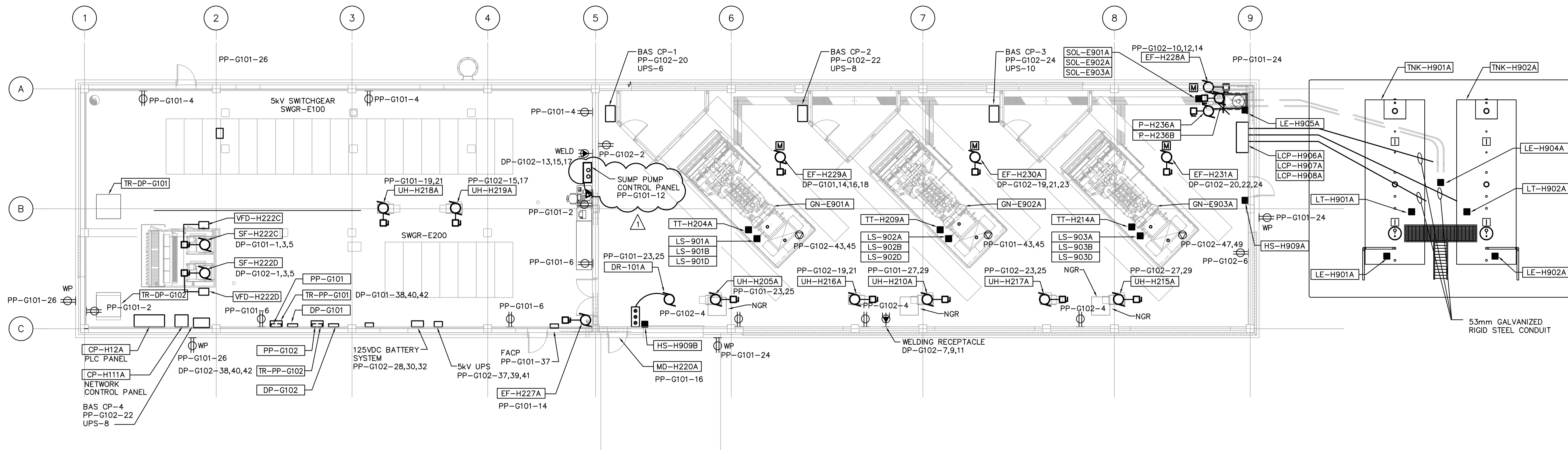
MAIN FLOOR PLAN
