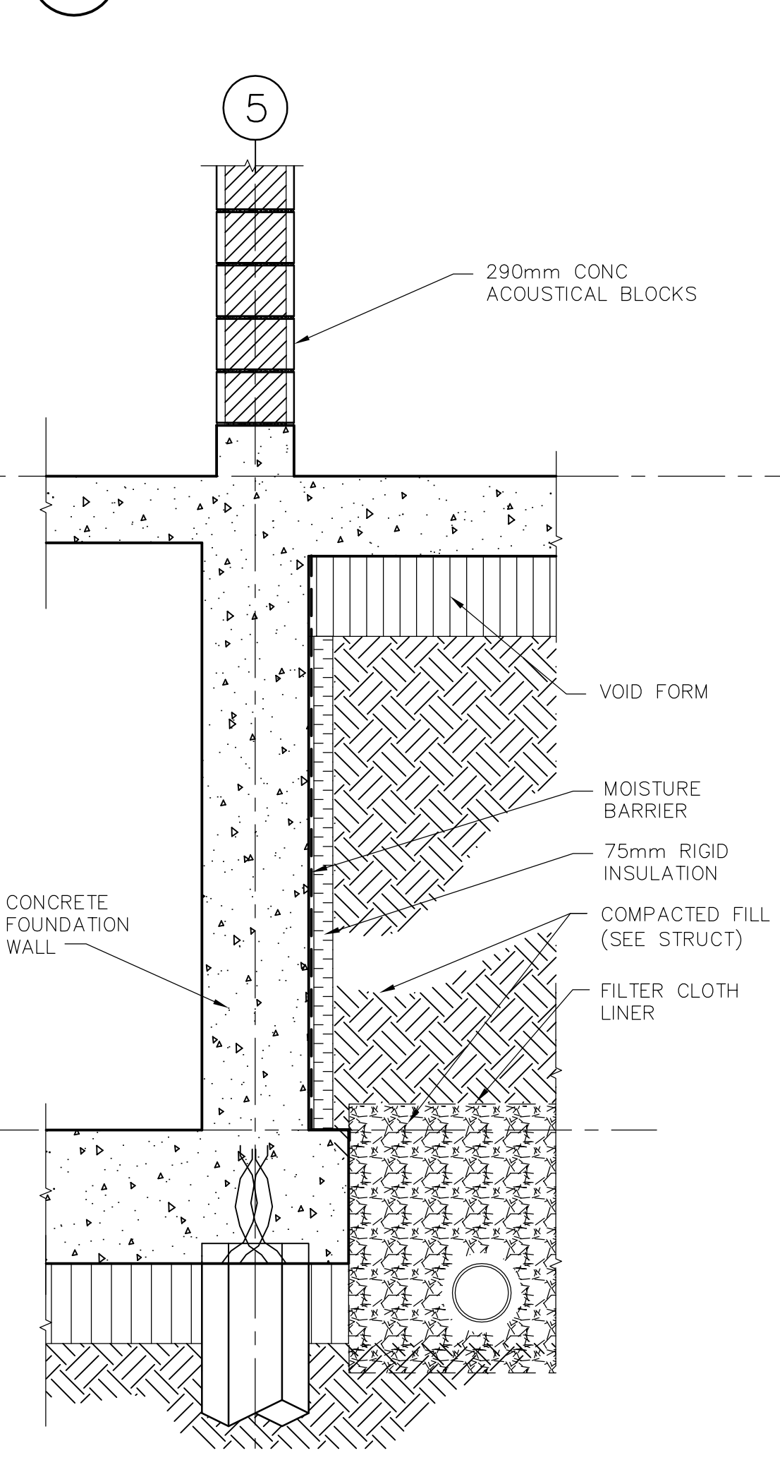
2 FOUNDATION WALL SECTION DETAIL WG-B0202 1:20
