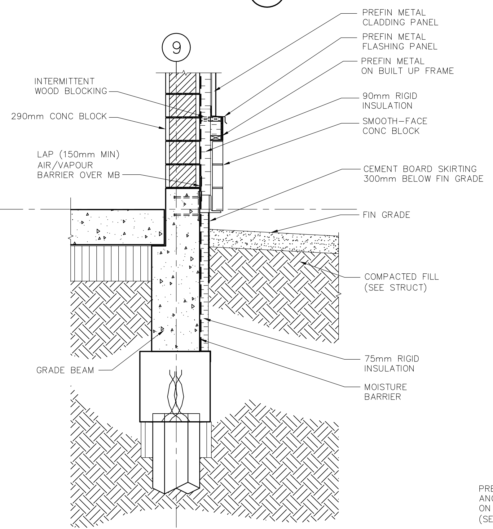
3 FOUNDATION WALL SECTION DETAIL WG-B0202 1:20
