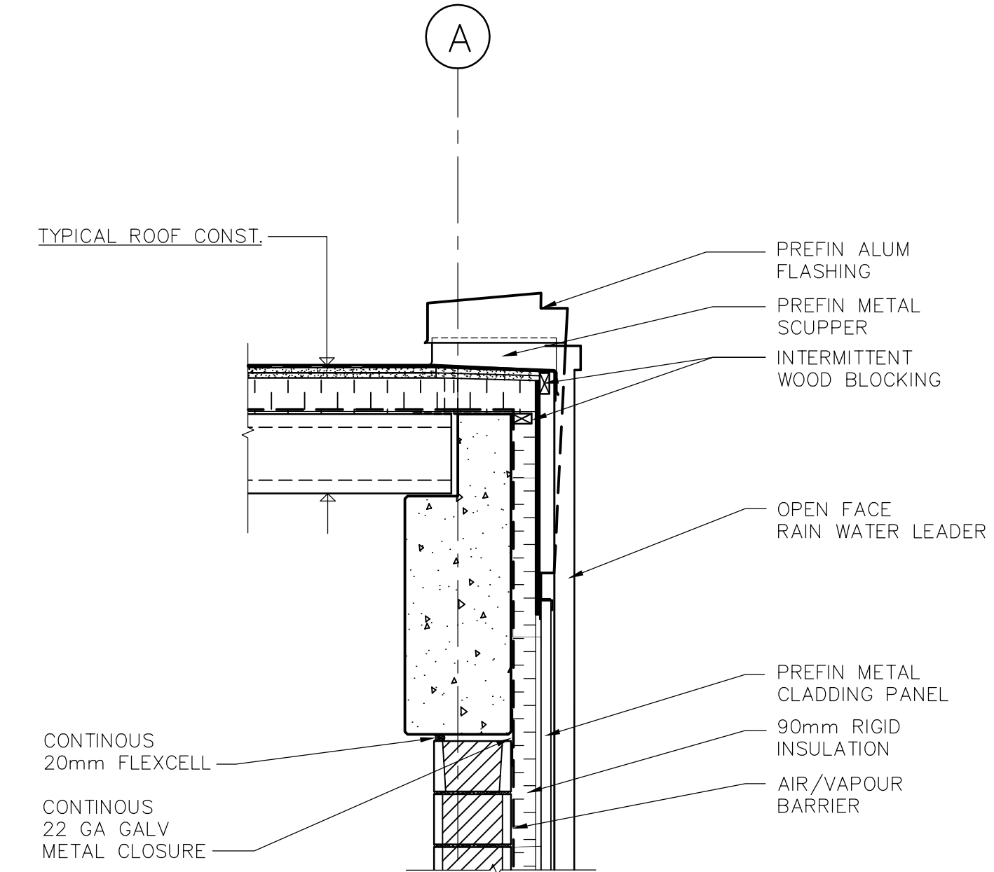
6 SCUPPER DETAIL WG-B0140 1:20
