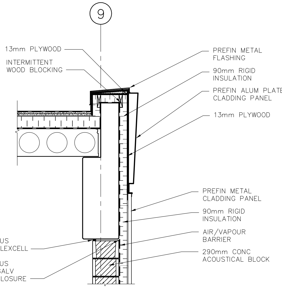
5 ROOF/WALL SECTION DETAIL WG-B0202 1:20
