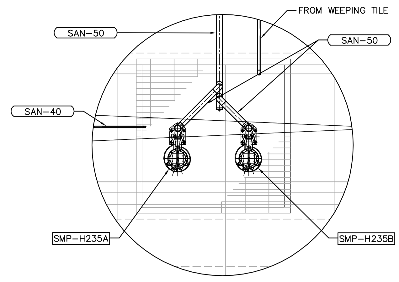
A SUMP PUMP PARTIAL PLAN 1:20
