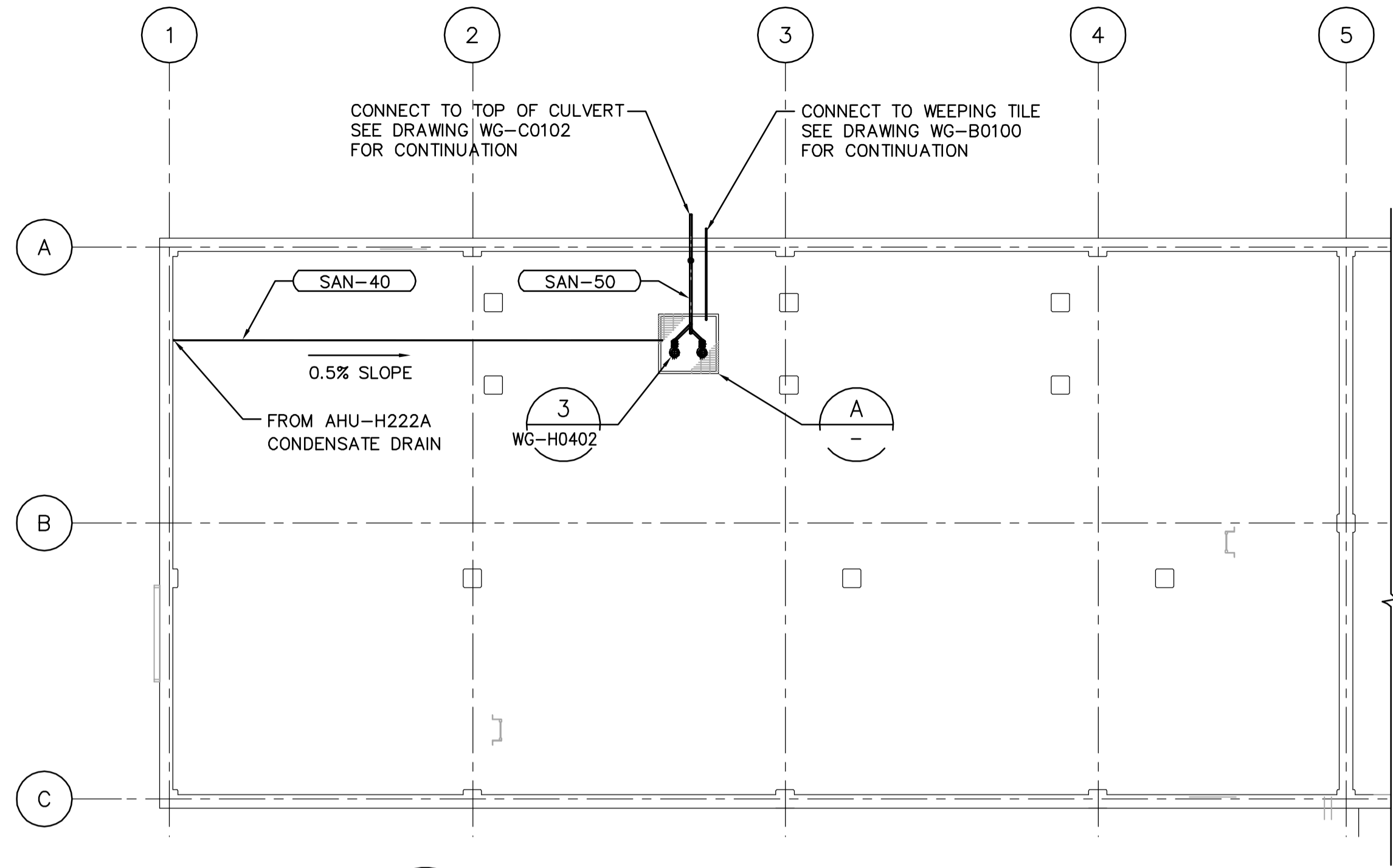
1 CRAWLSPACE PLUMBING PLAN WG-H0100 1:100
