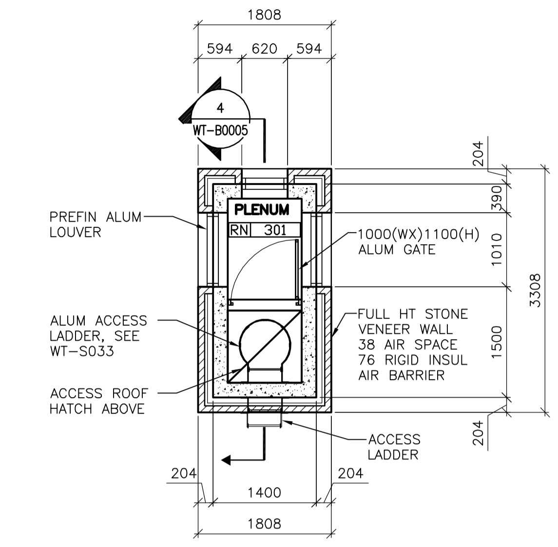
2 EMERGENCY EGRESS HUT FLOOR PLAN- TYPICAL OF 4 1:50
