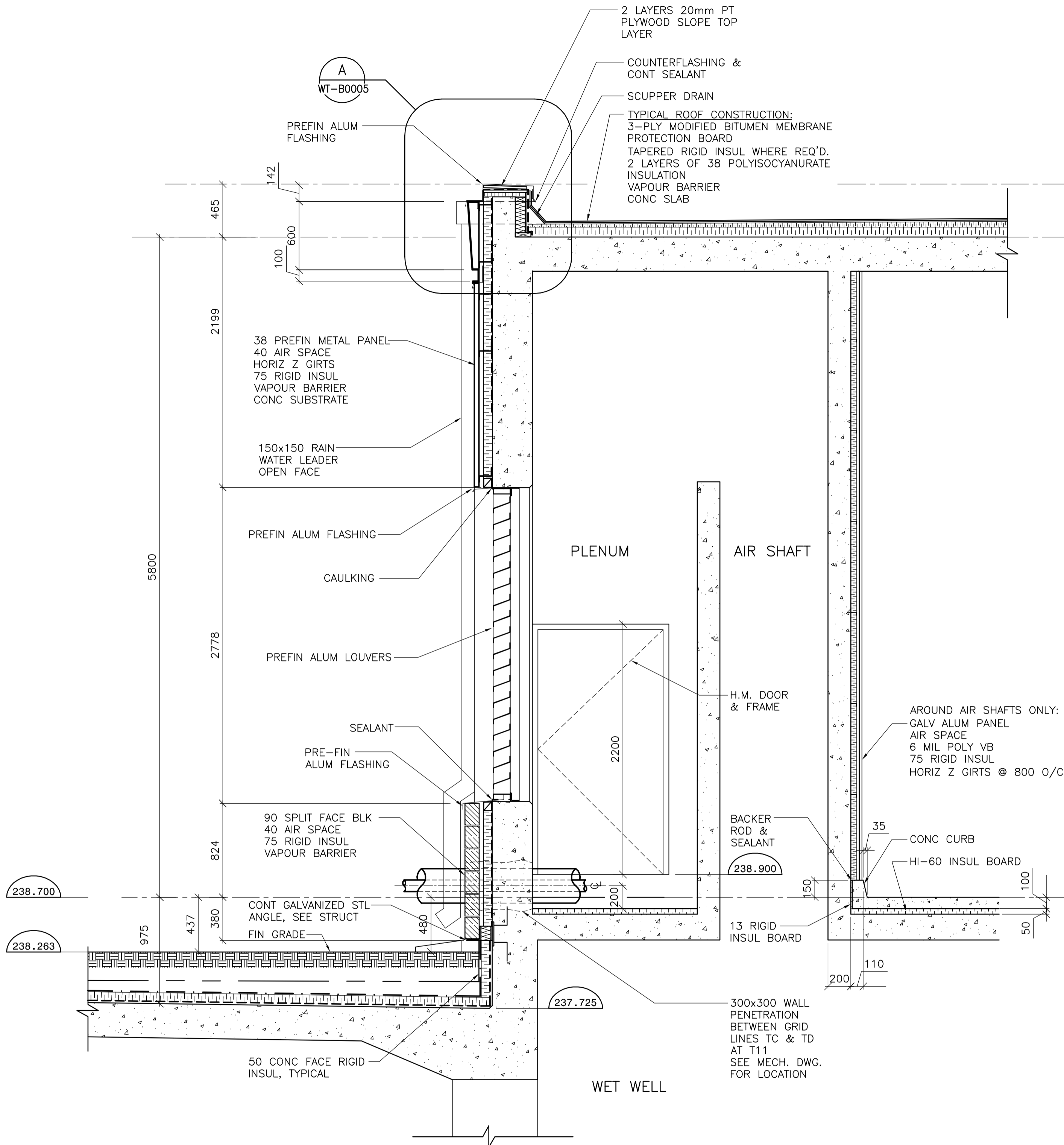
1 WALL SECTION DETAIL AT AIR SHAFT LOUVER WT-B0006 1:25
