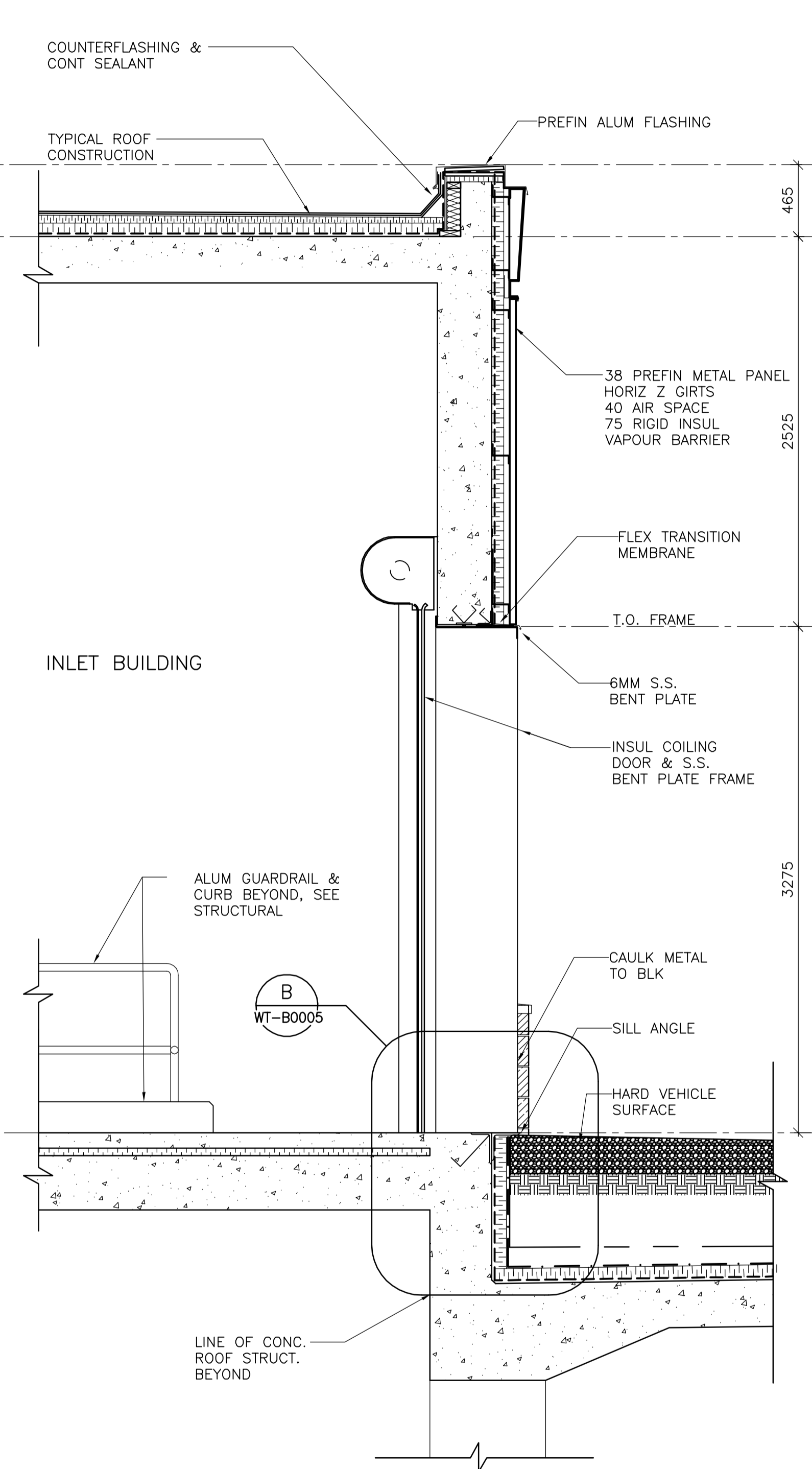
2 WALL SECTION DETAIL AT VERTICAL COILING DOOR WT-B0006 1:25
