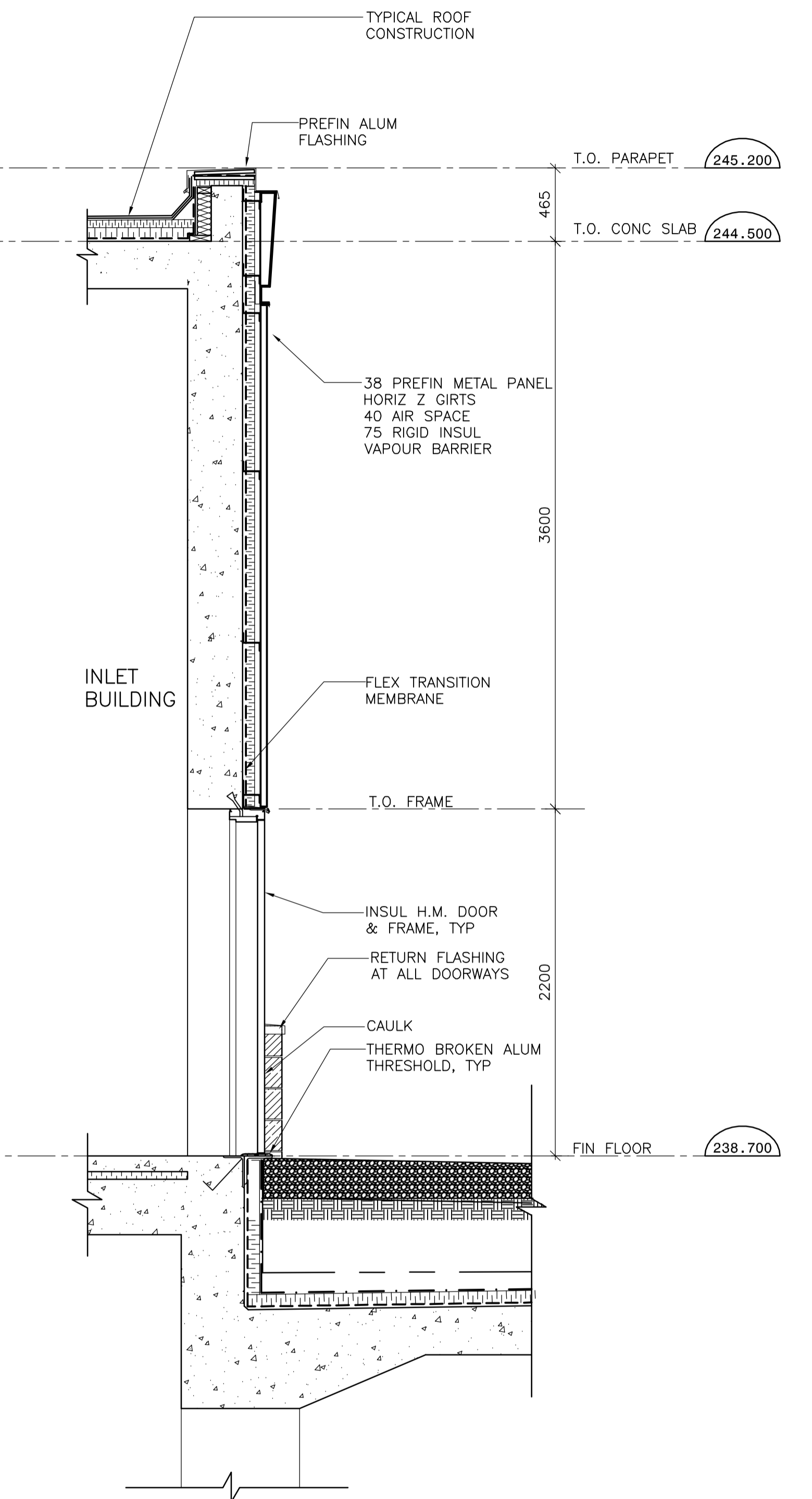
3 WALL SECTION DETAIL AT DOOR WT-B0002 1:25
