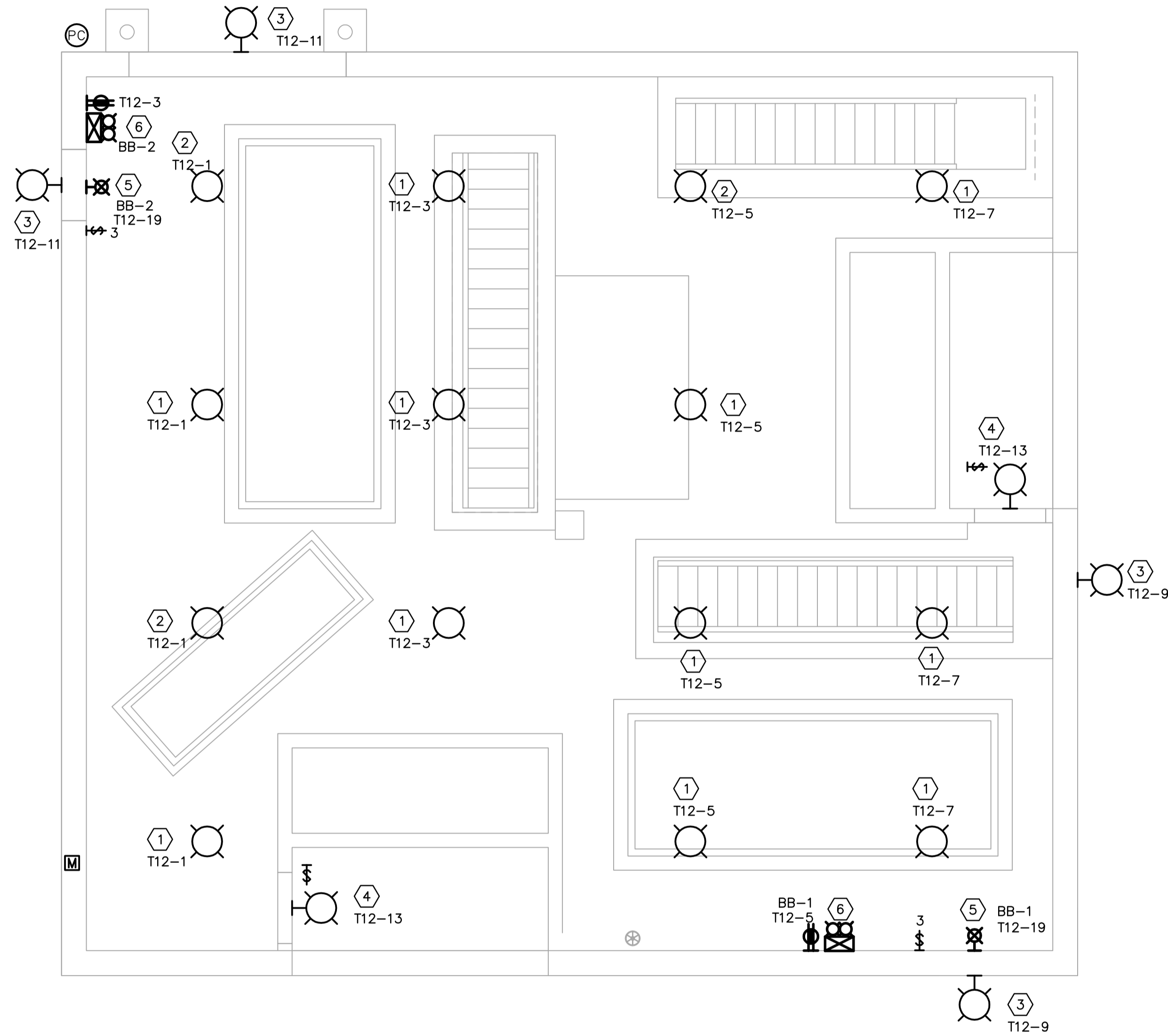
INLET BUILDING MAIN FLOOR LIGHTING PLAN 1:50
