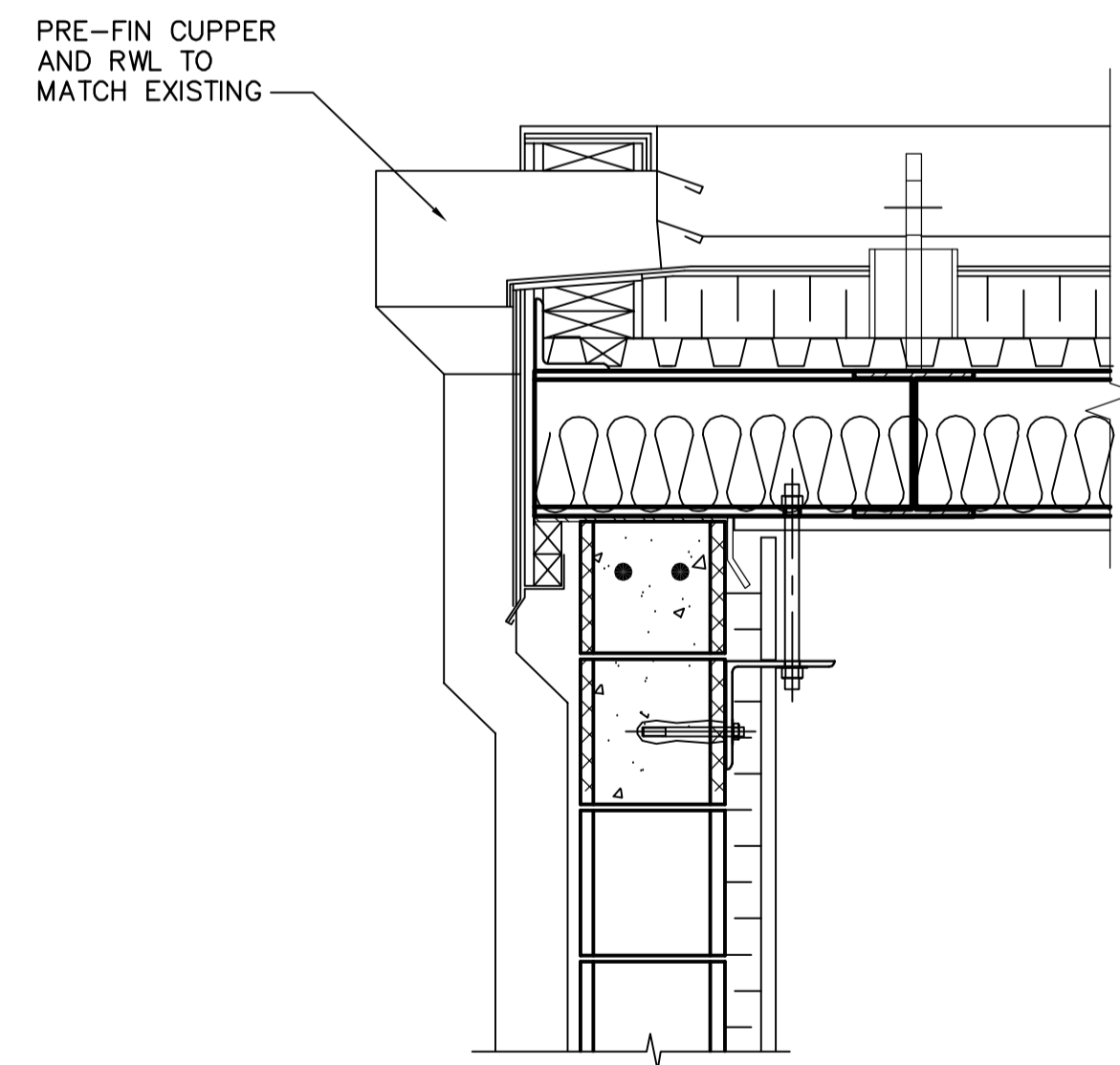
3 SCUPPER DETAIL WY-B0160 1:10
