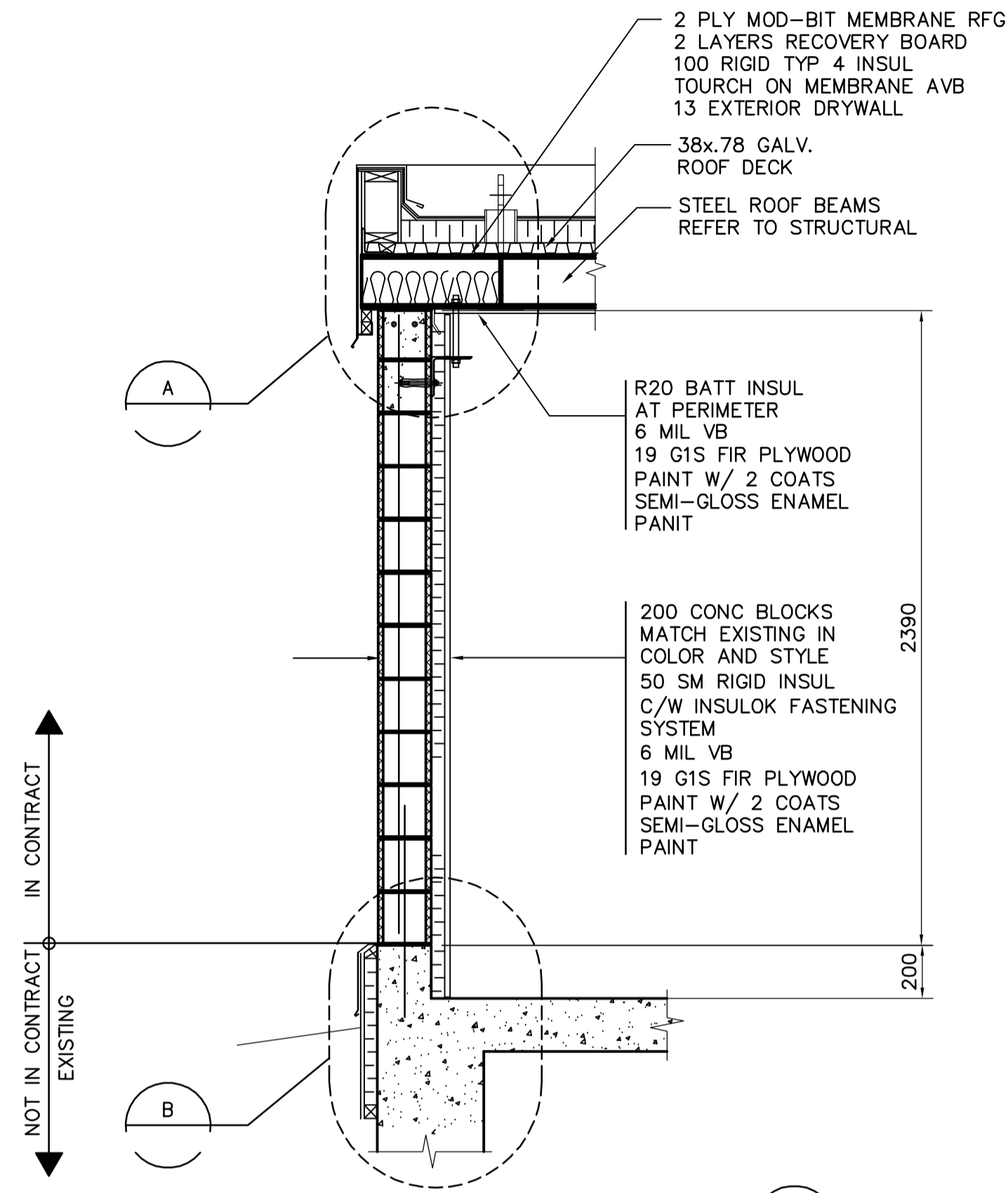
1 WALL SECTIONS WY-B0160 1:20
