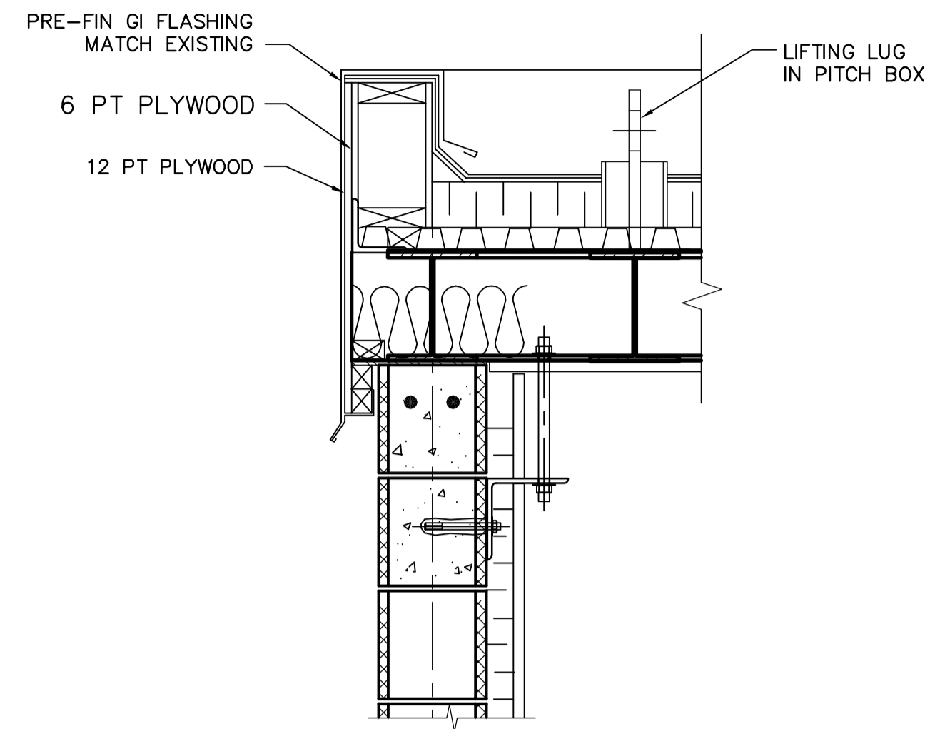
A DETAIL 1:10
