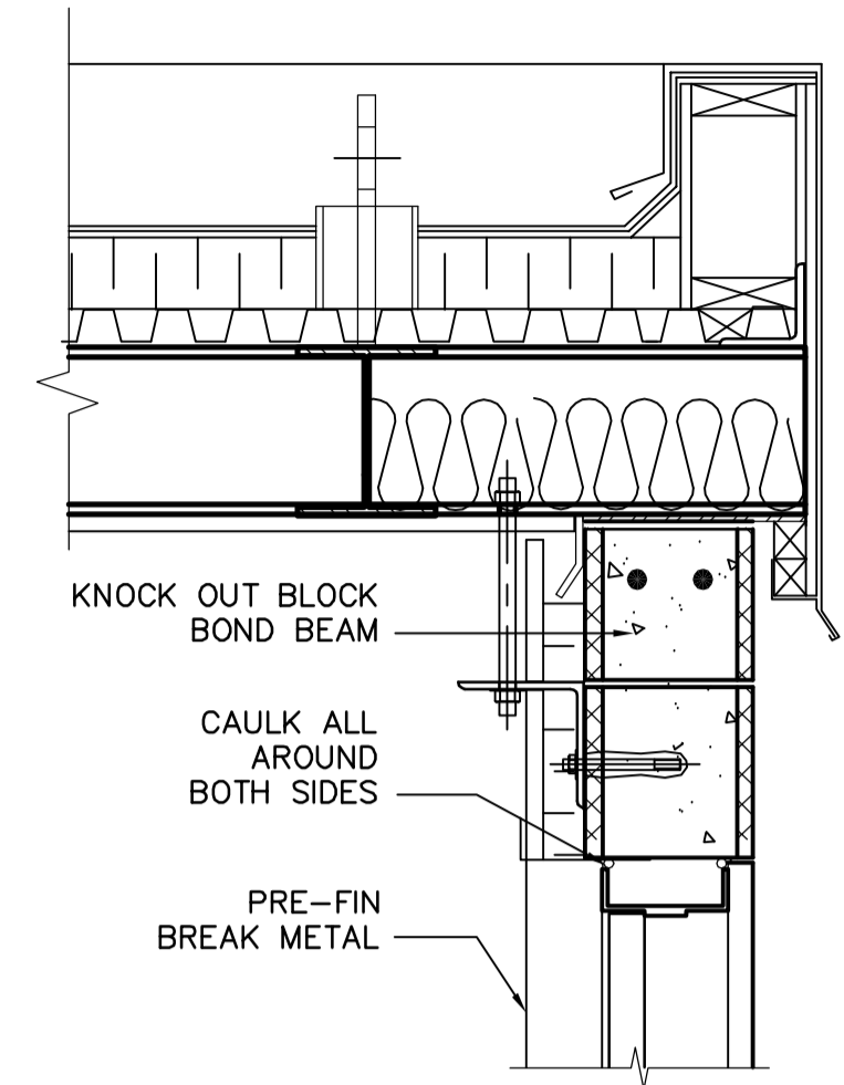
C DETAIL 1:10
