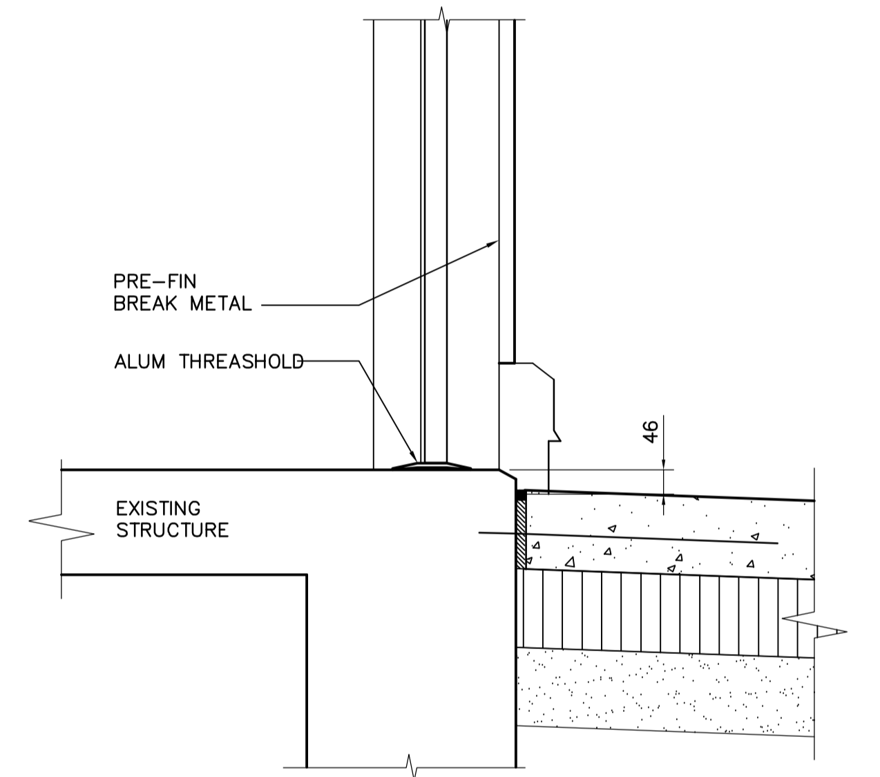
D DETAIL 1:10
