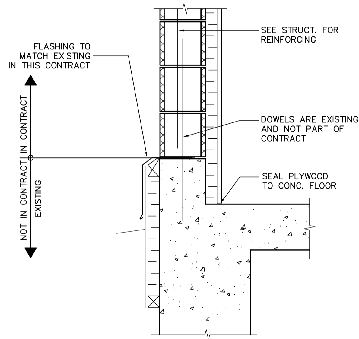
B DETAIL 1:10
