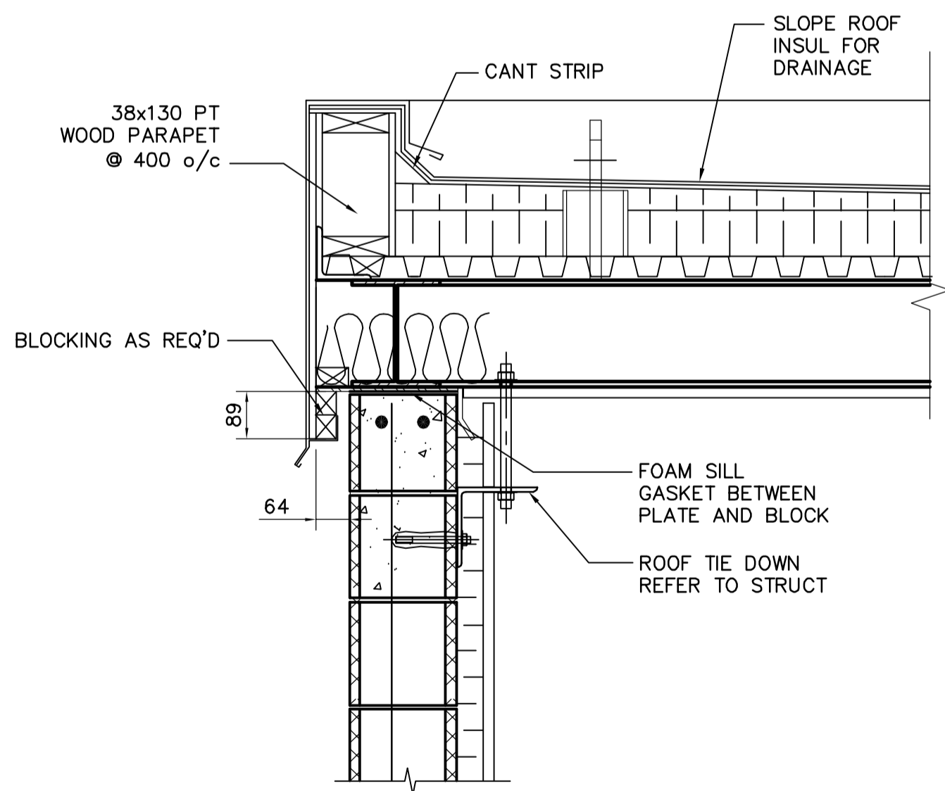
2 DETAIL WY-B0160 1:10
