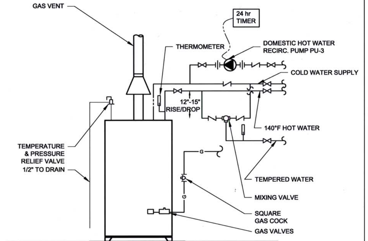
1 HOT WATER TANK DETAIL M1.3 SCALE: NTS
