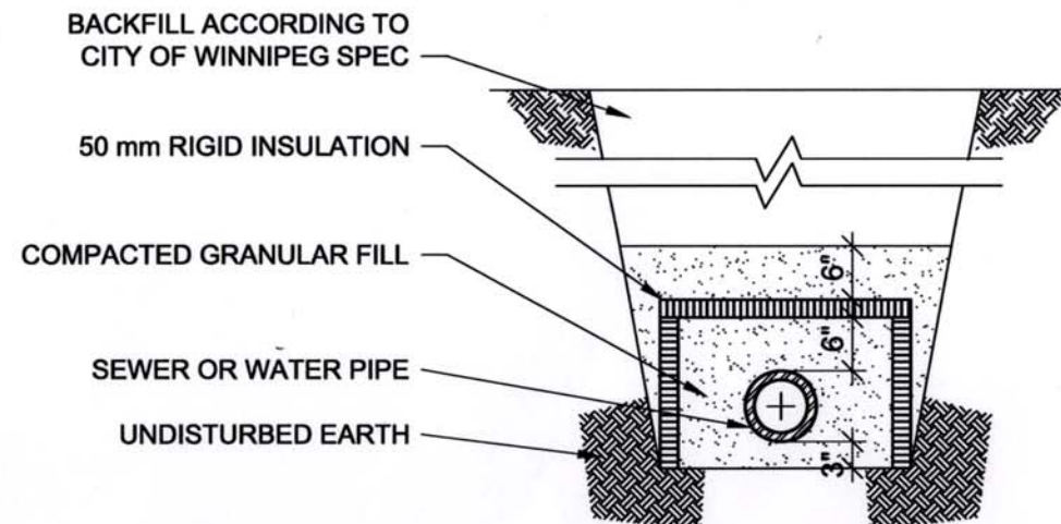
2 INSULATED WATER/SEWER SERVICE DETAIL M1.3 SCALE: N.T.S.
