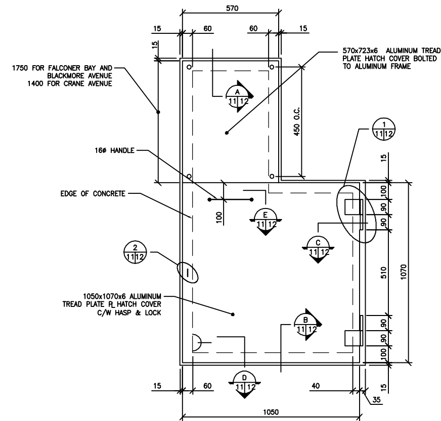
3 DETAIL 1:10
