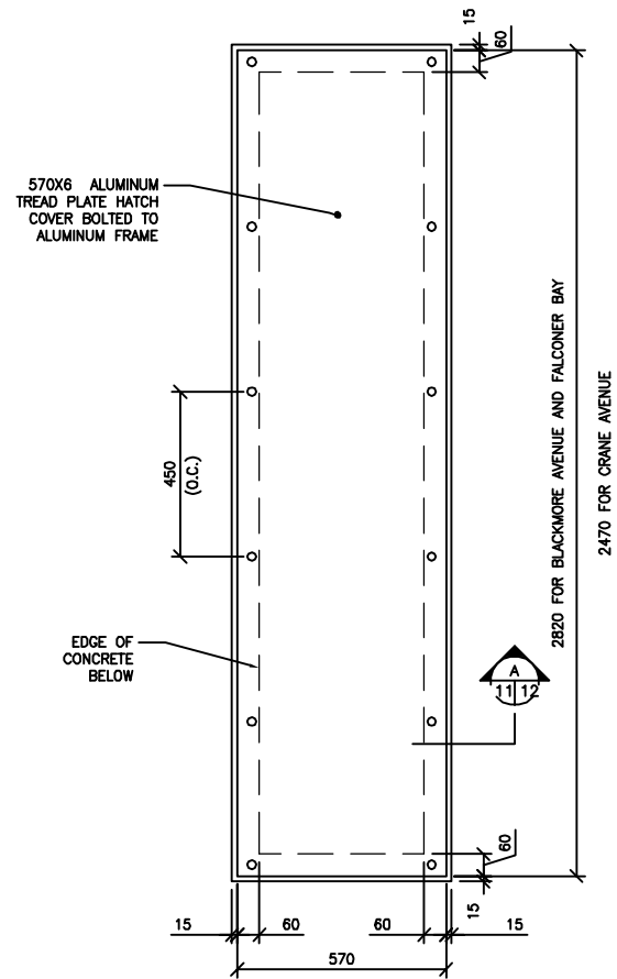
1 DETAIL 1:10
