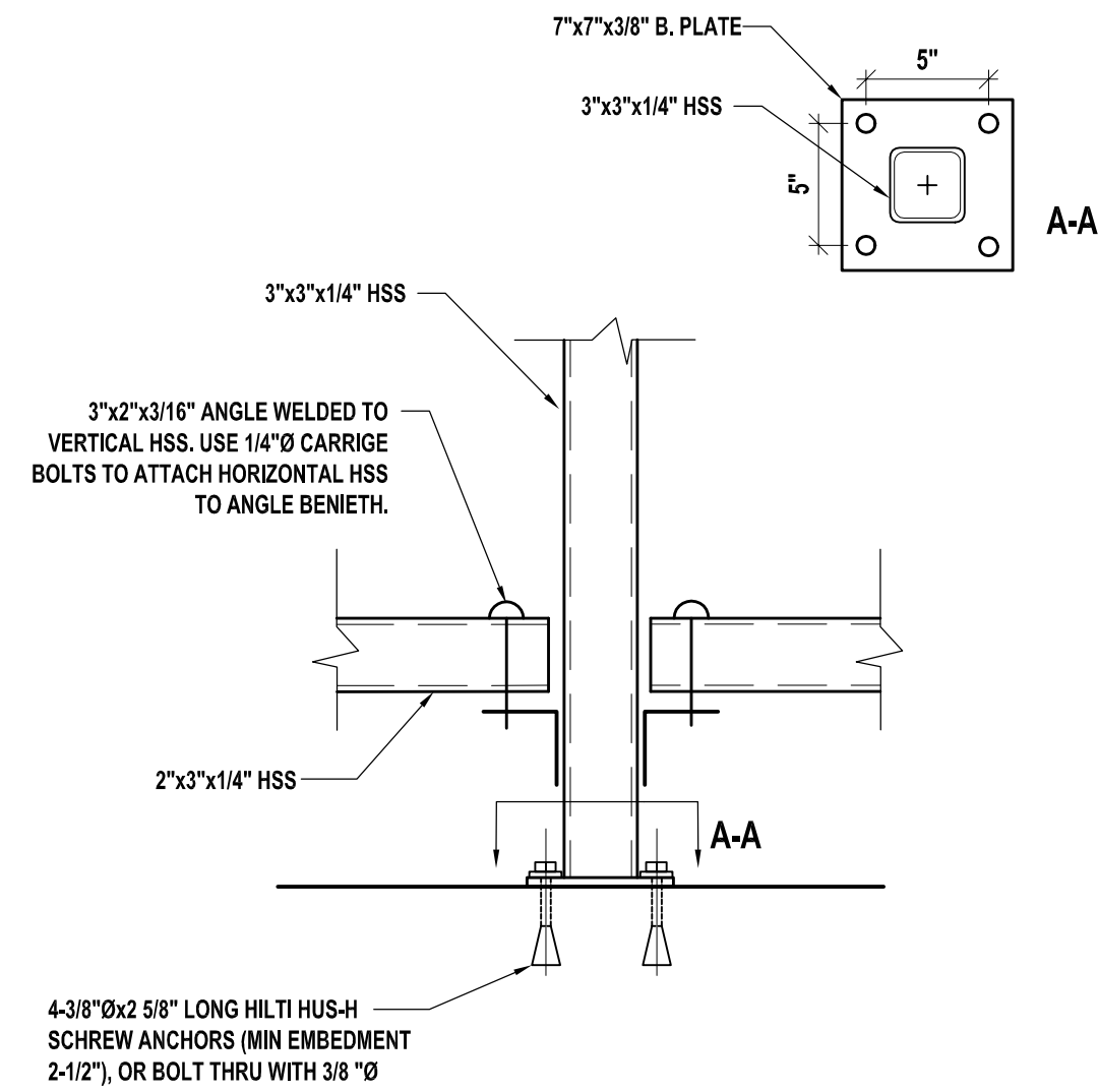
2 S1 S1 3"x3" HSS TO FLOOR CONNECTION (TYP) 1 1/2" = 1'-0"
