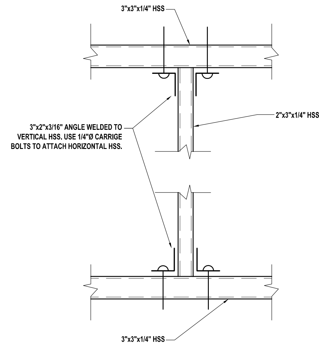
3 S1 S1 2"x3" HSS TO 3"x3" HSS CONNECTION (TYP) 1 1/2" = 1'-0"
