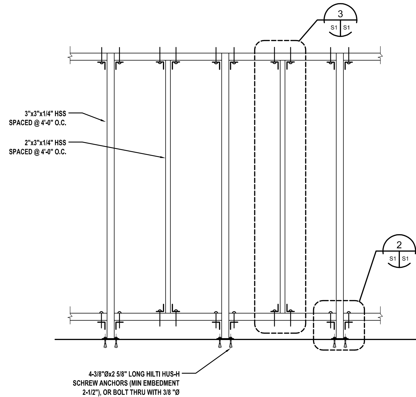
1 S1 S1 TYPICAL WALL ELEVATION 1/2" = 1'-0"
