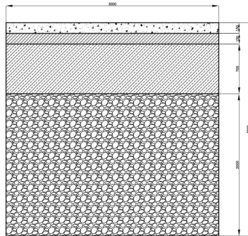
PROPOSED PAVEMENT SECTION
