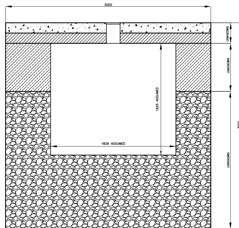
EXISTING PAVEMENT AND TANK SECTION
